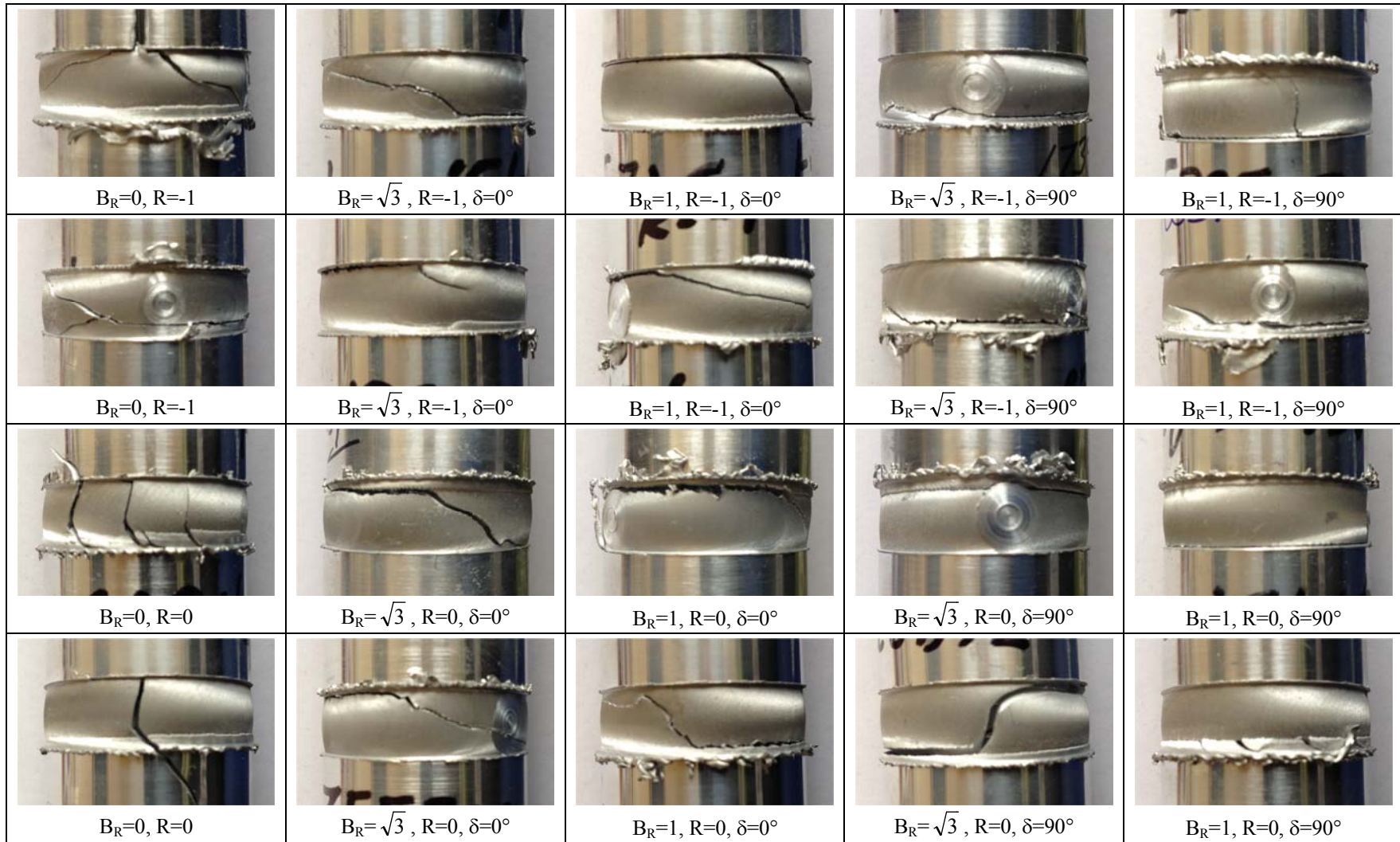
Figure 5. Examples of macroscopic cracking behaviour under biaxial cyclic loading.
