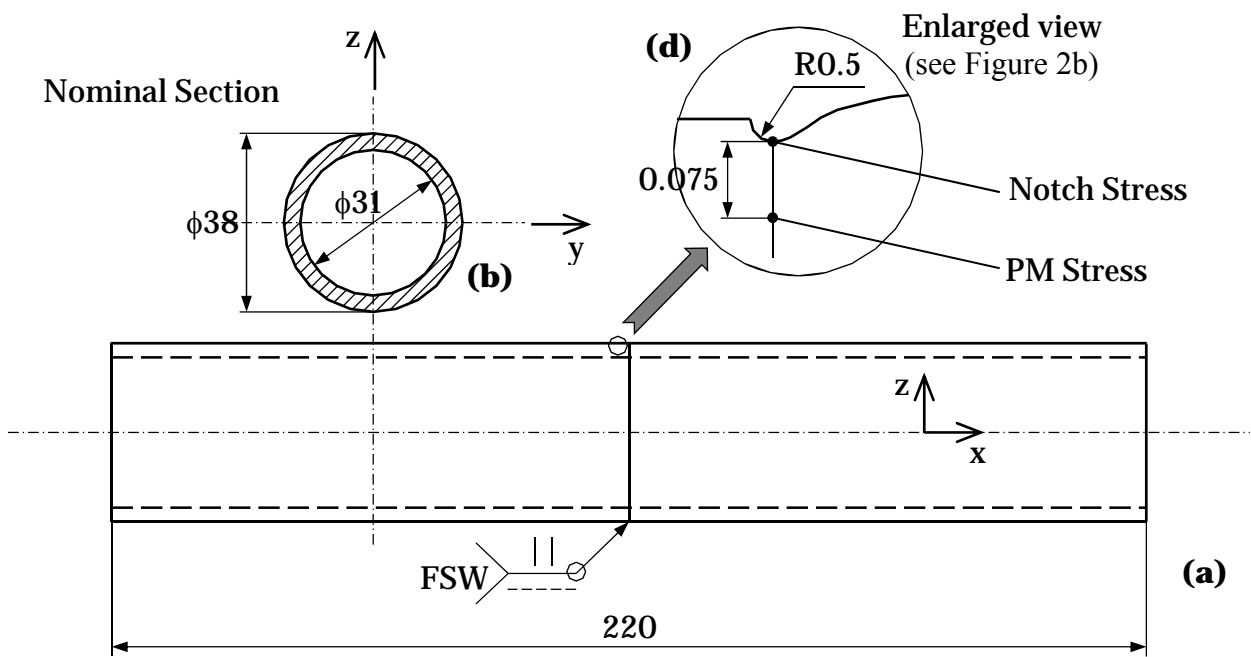
Figure 3. Technical drawing of the FS welded tubular specimen and adopted system of coordinates (dimensions in millimetres).
