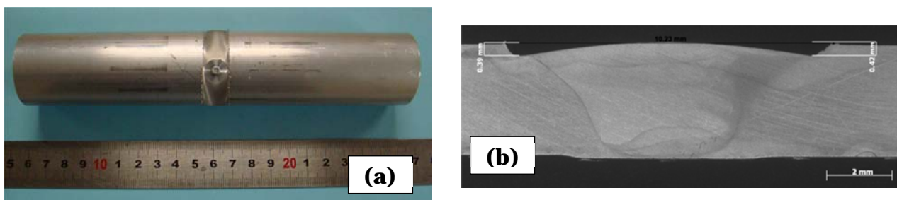
Figure 2. Al 6082-T6 FS welded tubular specimen (a); transverse macro-section of the weld region showing the notches resulting from the joining process (b).
