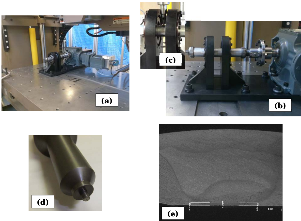
Figure 1. I-STIR FS welding platform equipped with a fourth axis (a); bearing supports with integrated clamping devices (b, c); welding tool developed to circumferentially FS weld tubes (d); example of transverse macro-section of the weld region (e).
