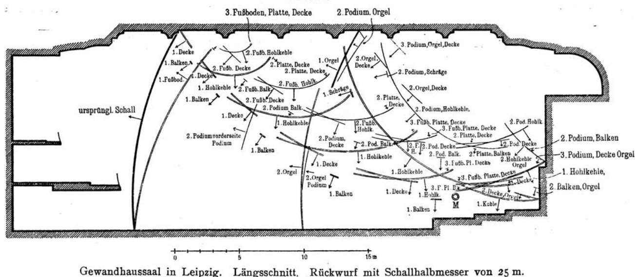
Figure 8 Eugen Michel, geometrical construction of sound propagation in the Gewandhausaal, Leipzig, 1921 (Eugen Michel, Hörsamkeit grosser Räume [Braunschweig: Vieweg, 1921], 32).
