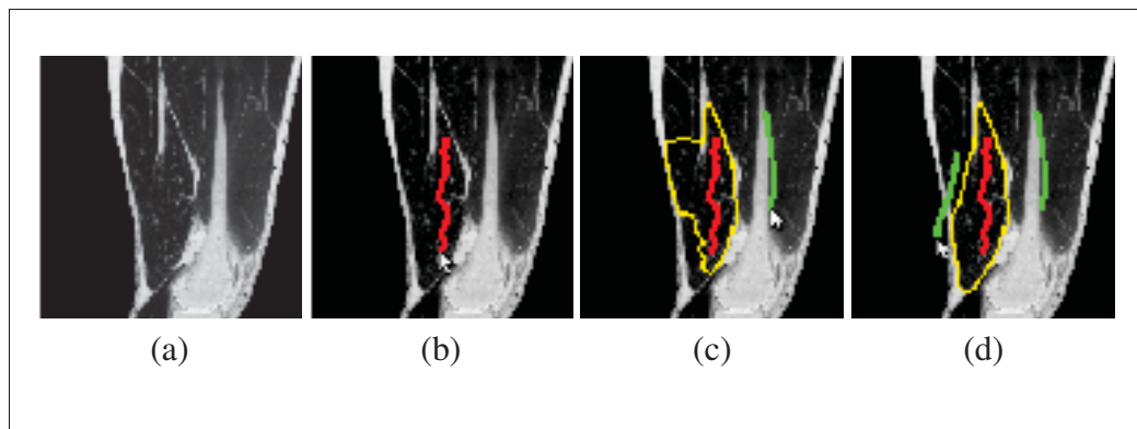
Figure 0.1 Example of scribble-based interactive segmentation: (a) the original image; (b-d) the user-drawn foreground (red) and background (green) labels yielding the computed segmentation (yellow)
