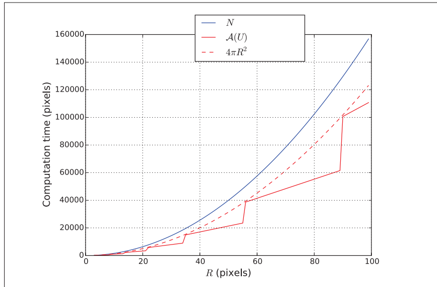
Figure-A I-2 Plot of N , A(U) , and 4\pi R^2 as a function of the radius R in pixels. Note that 4\pi R^2 = O(A(U))
