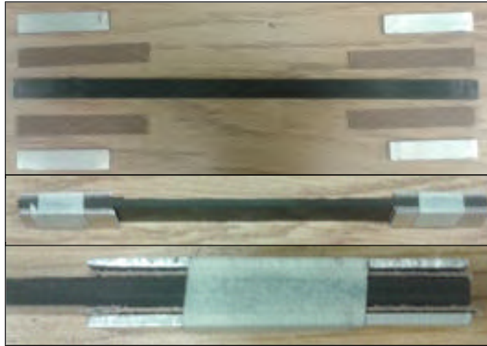
Figure 2.6: Sample with sandpaper and aluminium tabs
