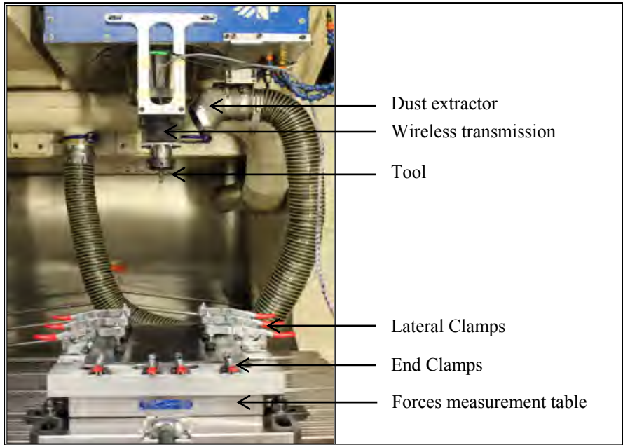
Figure 2.1: Machining setup
