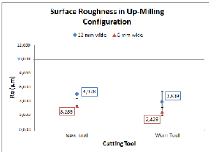
Figure 3.7: Surface roughness for both specimens width in up-milling configuration in function of the tool used
