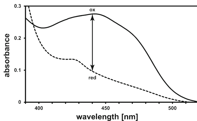
Fig. 2 Absorbance spectra of a cleared cell extract containing overexpressed BVMO. The spectra of the oxidised flavin cofactor in BVMO14 (continuous line) and after reduction by NADPH (broken line) are shown. The difference in absorbance at 440 nm that can be used to determine the BVMO concentration is indicated
