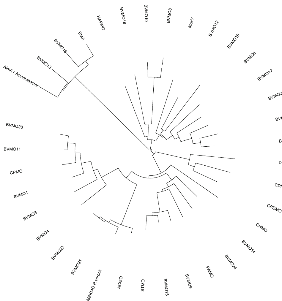
Fig. 1 Radial branching diagram of the comparison of active site residues of the selected BVMO protein sequences. The included sequences are: AlmA1 , Acinetobacter sp. DSM 17874 (ABQ18224.1); EtaA , Mycobacterium tuberculosis H37Rv (NP_218371.1); HAPMO , Pseudomonas fluorescens ACB (Q93TJ5.1); MoxY , Aspergillus flavus (AAS90037.1); PtIE , Streptomyces avermitilis MA-4680 (NP_824170.1); CDMO , Rhodococcus ruber SCI (AAL14233.1); CPDMO , Pseudomonas sp. strain HI-70 (BAE93346.1); CHMO , Acinetobacter calcoaceticus NCIMB 9871 (BAA86293.1); PAMO , T. fusca (YP_289549.1); STMO , Rhodococcus rhodochrous (BAA24454.1); ACMO , Gordania sp. strain TY-5 (BAF43791.1); MEKMO , Pseudomonas veronii MEK700 (ABI15711.1); CPMO , Comamonas sp. strain NCIMB 9872 (Q8GAW0)
