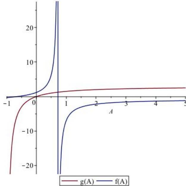
Figure 3.2: Non-Existence of a Positive Equilibrium
