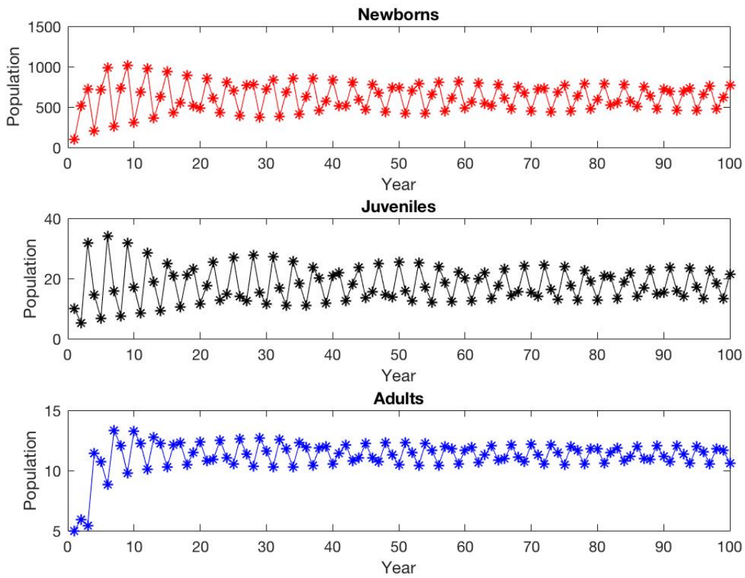
Figure 2.10: R_0 = 20 , b = 200 , high cannibalism
