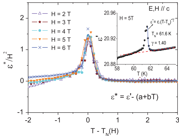
FIG. 7. (Color online) Dielectric constant scaled by H^2 plotted as a function of T - T_N(H) for E, H parallel to the c axis. The inset shows a fit to the divergence of the dielectric constant immediately above T_N , demonstrating critical behavior.
