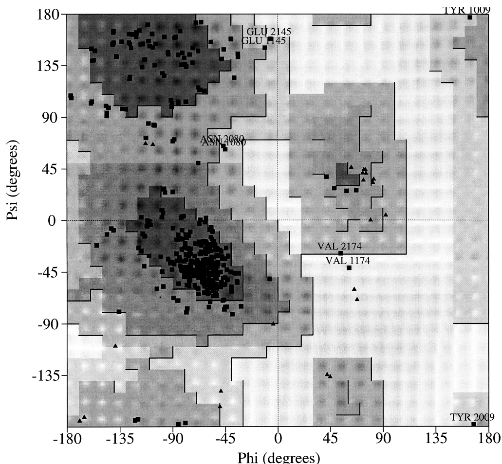
Fig. 2. Ramachandran plot as obtained from PROCHECK [41]. Val-174 of molecule A (named 1174) has unfavorable \phi, \psi angles. However, its conformation is well supported by electron density (real space correlation coefficient of OMIT map is 0.81).
