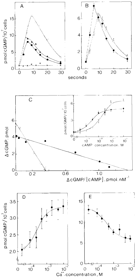
Fig. 7. The effect of \text{Ca}^{2+} on the cGMP-response. (A) Aggregative D. discoideum cells were stimulated with 100 nM cAMP at t = 0 s in the absence ( \circ ) or presence ( \bullet , \blacktriangle ) of 10 mM \text{Ca}^{2+} . Calcium ions were added at t = 5 s ( \blacktriangle ), or at t = -30 s ( \bullet ). In a control ( \times ), cells were not stimulated with cAMP, and \text{Ca}^{2+} was added at t = 0 s. (B) Cells were stimulated with 10 nM cAMP at t = 0 s in the absence ( \circ ) or presence of 10 mM \text{Ca}^{2+} ( \bullet ). \text{Ca}^{2+} was added at t = -30 s. (C) Cells were lysed at 5 s after stimulation with different cAMP concentrations. ( \circ ), control cells; ( \bullet ), cells preincubated with 10 mM \text{Ca}^{2+} for 30 s. The inset is a dose response-curve. The main figure is an Eadie-Hofstee plot of the same data; \Delta\text{cGMP} represents the increase in cGMP levels. (D) Cells were preincubated with different \text{Ca}^{2+} concentrations for 30 s, then stimulated with 5 nM cAMP and lysed at 5 s after stimulation. (E) Cells were preincubated with different \text{Ca}^{2+} concentrations for 30 s, then
