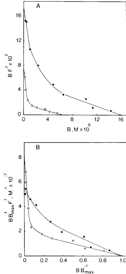
Fig. 4. The effect of \text{Ca}^{2+} on the Scatchard plot of H+L. D. discoideum cells were incubated with different [^3\text{H}]\text{cAMP} concentrations in the absence ( \circ ) or presence ( \bullet ) of 10 mM \text{Ca}^{2+} . Cell-associated radioactivity was determined after an incubation period of 45 s, and is bound to the three cAMP-binding sites, H, L and S (part A). At 6 s after a chase with excess cAMP, essentially all cell-associated cAMP is bound to S. During this 6 s chase, about 25% of the occupied S-sites dissociate; therefore the occupation of S at 45 s equals the occupation after a 6 s chase (Fig. 3) divided by 0.75. This value is subtracted from total binding at 45 s (Fig. A), whereby the binding to H+L is obtained. These data are presented in part B. Data were normalized for differences in B_{\text{max}} to obtain a better impression of the differences in linearity of the two curves.
