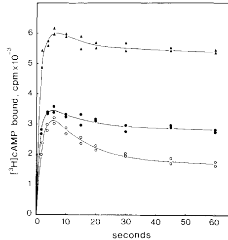
Fig. 1. The effect of \text{Ca}^{2+} on the association of cAMP to D. discoideum cells. Cells were rapidly mixed with 30 nM [ ^3\text{H} ]cAMP (about 100000 cpm) in the absence ( \circ ) or presence of 30 \mu\text{M} \text{Ca}^{2+} ( \bullet ) or 1 \text{ mM} \text{Ca}^{2+} ( \blacktriangle ). At the times indicated, cell-associated [ ^3\text{H} ]cAMP and free [ ^3\text{H} ]cAMP were separated by centrifugation of the cells through silicon oil in a small swing-out rotor at 10000 \times g for 15 s. Nonspecific binding, which was determined by including 100 \mu\text{M} cAMP in the incubation mixture, was subtracted from all data shown.
