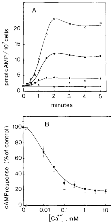
Fig. 6. The effect of Ca^{2+} on cAMP relay. (A) Aggregative D. discoideum cells were stimulated with 10 \mu M cdAMP and 5 mM dithiothreitol in the absence (○) or presence of 30 \mu M (●) or 1 mM (▲) Ca^{2+} . In a control (×), cells were not stimulated with cdAMP or dithiothreitol; to these cells was added 1 mM Ca^{2+} . At the times indicated, cells were lysed and the cAMP content was measured by isotope dilution assay in which cdAMP did not show cross-inhibition; (B) cAMP content at 3 min after stimulation of aggregative cells with cdAMP and dithiothreitol in the presence of different Ca^{2+} concentrations.
