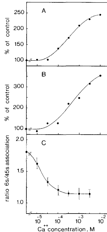
Fig. 5. Dose-response curves of the effect of \text{Ca}^{2+} on B_{\text{max}} (A); the affinity of S (B); and the transition of H to L (C). (A) cells were incubated with 200 nM [ ^3\text{H} ]cAMP in the presence of different \text{Ca}^{2+} concentrations for 45 s. Binding in the absence of added \text{Ca}^{2+} was 400 \pm 26 \text{ fmol}/10^7 \text{ cells} ( n = 4 ). (B) cells were incubated with 1 nM [ ^3\text{H} ]cAMP in the presence of different \text{Ca}^{2+} concentrations for 45 s. Then excess cAMP was added, and cell-associated [ ^3\text{H} ]cAMP was measured 6 s later. Binding in the absence of added \text{Ca}^{2+} was 3 \pm 0.1 \text{ fmol}/10^7 \text{ cells} , ( n = 4 ). (C) Cells were incubated with 30 nM [ ^3\text{H} ]cAMP in the presence of different \text{Ca}^{2+} concentrations for 6 s and for 45 s. The ratio of cell-associated [ ^3\text{H} ]cAMP after these incubation periods is presented.
