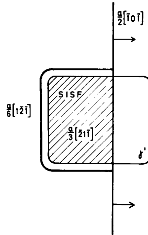
Fig. 5. Growth mechanism of stacking faults inside \gamma' precipitates.
