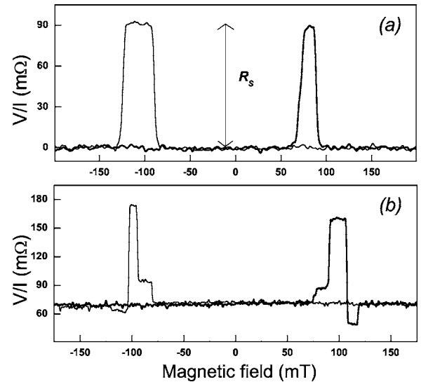
FIG. 2. Nonlocal spin valve measurement: the transresistance V/I as a function of the in-plane magnetic field for positive and negative sweep direction. (a) Device A, two switch traces of the cobalt electrodes and (b) Device B, four switch traces, at low temperature (2 K).
