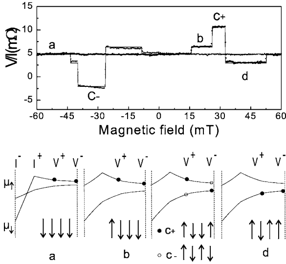
FIG. 3. (Top) Experimental data (dots) and fitting results (lines) using Eq. (1) for nonlocal spin valve at room temperature, device C. The letters a to d represent the different magnetic configurations as described below. (Bottom) Spatial dependence of \mu_{\uparrow} and \mu_{\downarrow} electrochemical potentials in the Al island for the magnetic configurations a to d , as in the top panel. The filled (open) dots indicate the potential measured by the V^+ and V^- probes.
