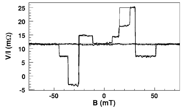
FIG. 4. Nonlocal spin accumulation at room temperature, device D. The fitting based on Eq. (1) returns \lambda_{sf} = (350 \pm 50) nm and a polarization of P = (8 \pm 1)\% .
