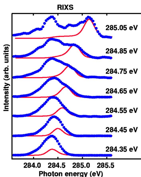
FIG. 4. (Color online) RIXS data (dotted lines) taken at photon energies similar to the RPES data. The position of the elastic peak is indicated by a Gaussian (solid lines) centered at the incident photon energy. In the lowest three spectra the intensity of the elastic peak is estimated by the constraint that the result of subtracting the elastic peak should not induce structures not already apparent in the raw data.
