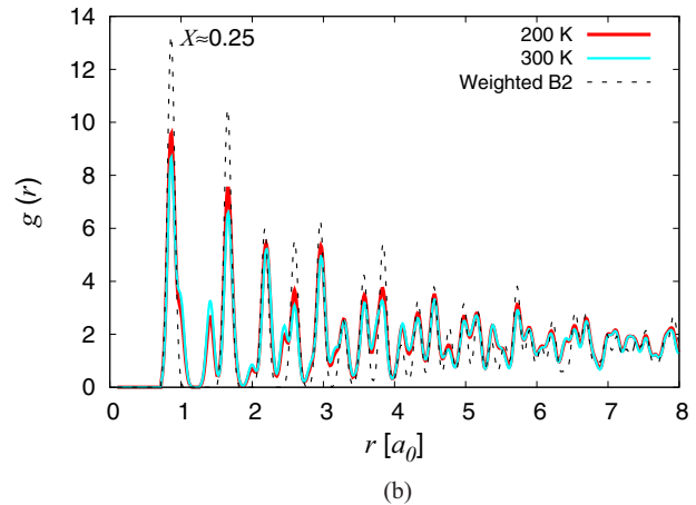
FIG. 17. Atomistic snapshots of the equilibrium configurations of the W-25Re system and associated pair correlation function at 200 and 300 K. (a) X \approx 0.25 . (b) Pair correlation function.
