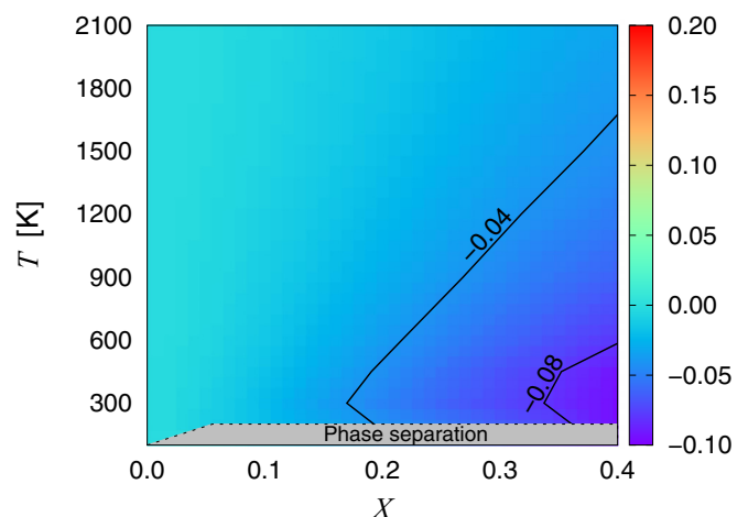
FIG. 6. Structural phase diagram showing regions of changing SRO. The dashed lines are the limits of applicability of the rigid bcc lattice model. The system displays slightly negative SRO throughout the entire temperature-concentration space, indicating a preference to be in a solid solution state. The gray band at low temperatures signifies the region of coexistence of the bcc and B2 phases (see Appendix A).
