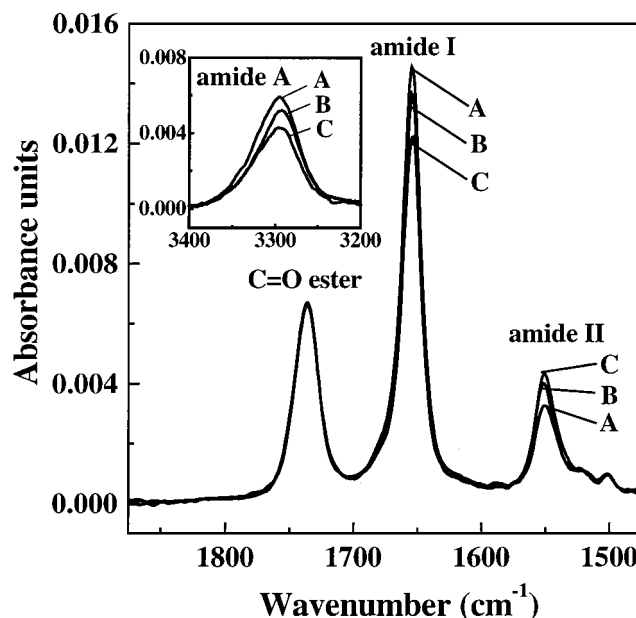
Figure 4. FT-IR transmission spectra of (A) a PBLG LB assembly of 10 monolayers, (B) the grafted PBLG layer with the smallest average angle between the helices and the substrate, and (C) the grafted PBLG layer with the largest average angle of the helices.
