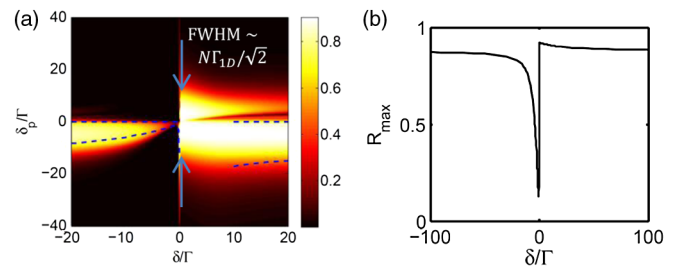
FIG. 4 (color online). (a) Reflectance from self-organized atomic configuration versus pump ( \delta ) and probe ( \delta_p ) detunings. The dashed blue curves indicate the edges of the band gap region \delta_{\text{gap}} , which is well defined when a single lattice constant exists (i.e., outside of the phase slip configuration). The lattice constant used here is the average over all atoms. For the phase slip configuration, the reflectance spectrum is nearly symmetric with respect to \delta_p , with a FWHM given by \sim N\Gamma_{\text{ID}}/\sqrt{2} . (b) Maximum reflectance (optimized with respect to \delta_p ) versus pump detuning. All simulations are for N = 150 atoms and \Gamma_{\text{ID}}/\Gamma = 0.25 .
