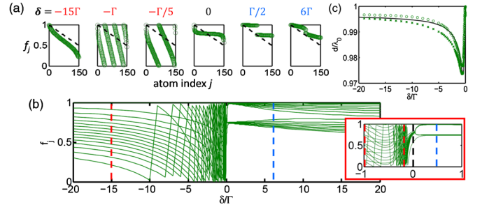
FIG. 2 (color online). (a) Fractional positions f_j versus atom index for selected pump detunings \delta/\Gamma = -15, -1, -0.2, 0, 0.5, 6 . All numerical simulations are for N = 150 atoms and \Gamma_{1D} = \Gamma/4 . The dotted line represents the solution in the weak-scattering limit. (b) Positions f_j versus pump detuning. The vertical dashed lines denote the detunings for which the positions are plotted in (a). For clarity, only 16 representative atomic positions are shown here. Inset: zoom of the same plot near \delta/\Gamma = 0 . (c) Characteristic lattice constant d/\lambda_0 versus detuning for \delta < 0 . The circles and crosses denote the lattice constant as determined by the central two atoms and the average over all atoms, respectively. The solid curve depicts d_{\text{eff}} = \lambda_{\text{eff}}(1 - 1/2N) , where \lambda_{\text{eff}} accounts for the effective refractive index provided by the atomic medium.
