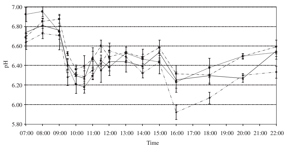
Figure 1 Rumen pH of beef steers given diets based on forage mixtures of grass and maize silage ( \circ = G, \bullet = GGM, \blacktriangle = MMG, \diamond = M).
