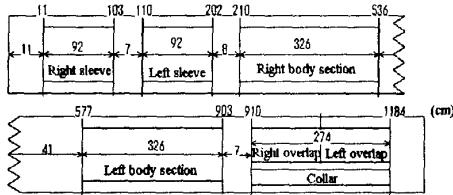
Fig. 16. The cutting pattern of the striped yukata
