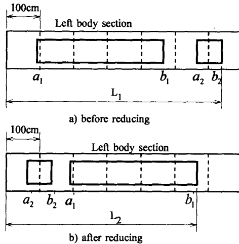
Fig. 13. Undesirable designs
