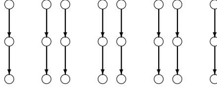
Figure 6.4: A BT-structure
