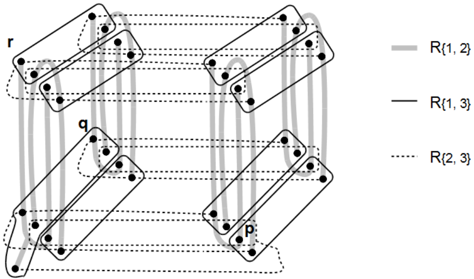
Figure 8.1: A NCL-model for \neg[\langle\{2,3\}\rangle p \wedge \langle\{1,3\}\rangle q \wedge \langle\{1,2\}\rangle r \rightarrow \langle\emptyset\rangle[\langle\{2,3\}\rangle(\langle\{1,3\}\rangle p \wedge \langle\{2,3\}\rangle q) \wedge \langle\{1,3\}\rangle(\langle\{2,3\}\rangle r \wedge \langle\{1,2\}\rangle p) \wedge \langle\{2,3\}\rangle(\langle\{1,2\}\rangle q \wedge \langle\{1,3\}\rangle r)]]
