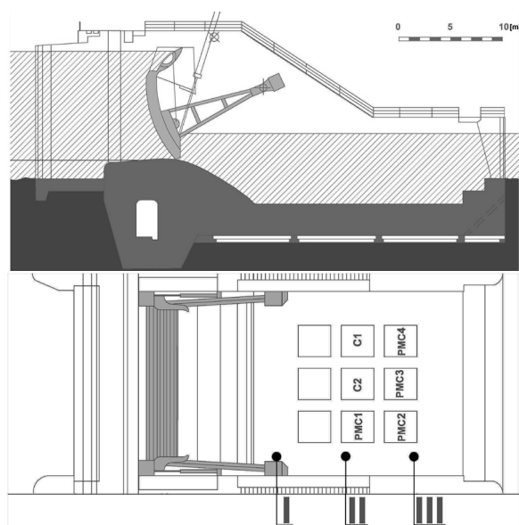
Fig. 1. Location of test plots and the control profiles of base concrete in the stilling basin of the Vrhov HPP spillway
