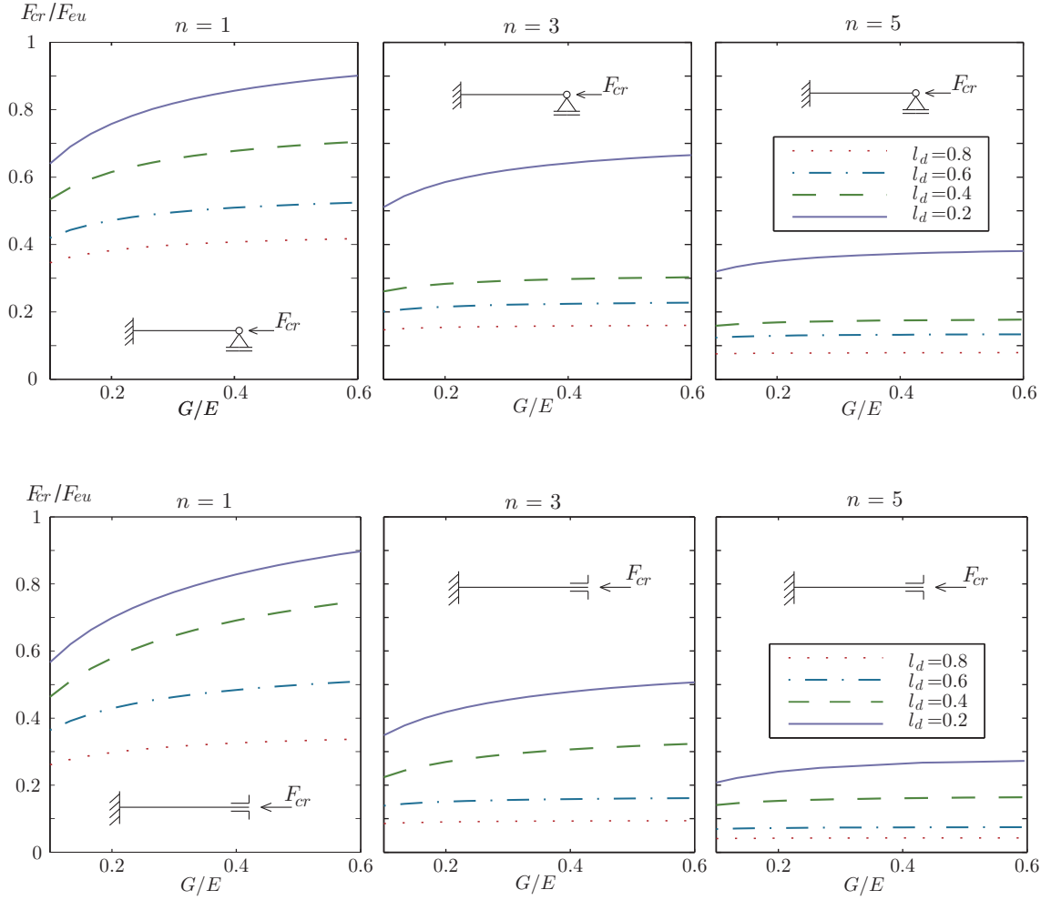
Fig. 7. Effect of transverse shear on the normalized buckling load for the clamped-pinned and the clamped-clamped beams with 1, 3 and 5 delaminations of various lengths, l_d .
