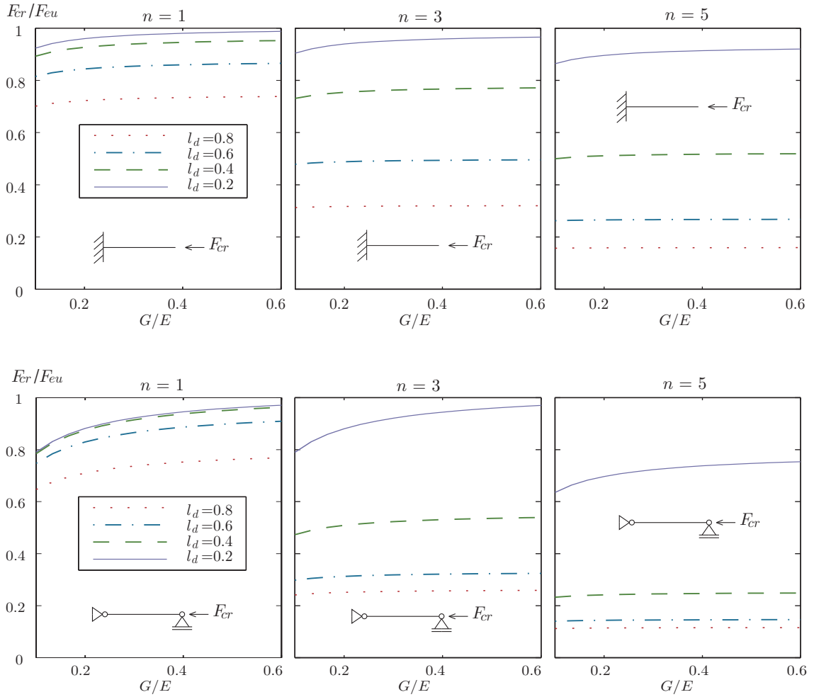
Fig. 6. Effect of transverse shear on the normalized buckling load for the cantilever and the simply supported beam with 1, 3 and 5 delaminations of various lengths.
