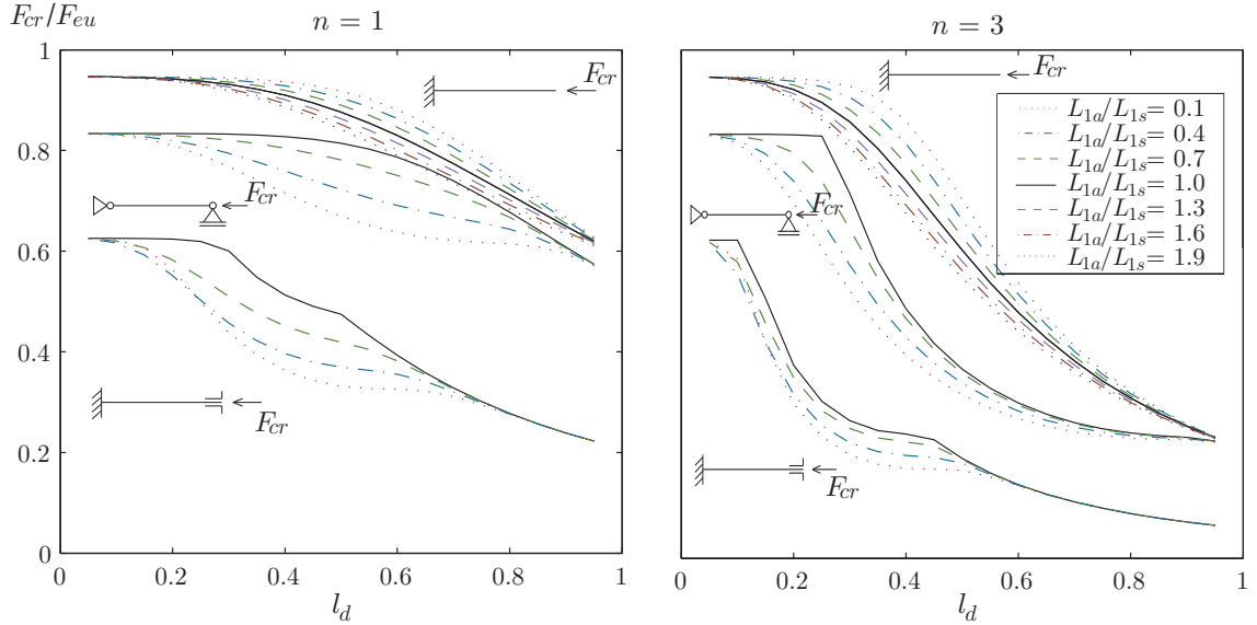
Fig. 13. Effect of longitudinal asymmetry on the normalized buckling load for the clamped-clamped beam, the simply supported beam and the cantilever with one or three delaminations.
