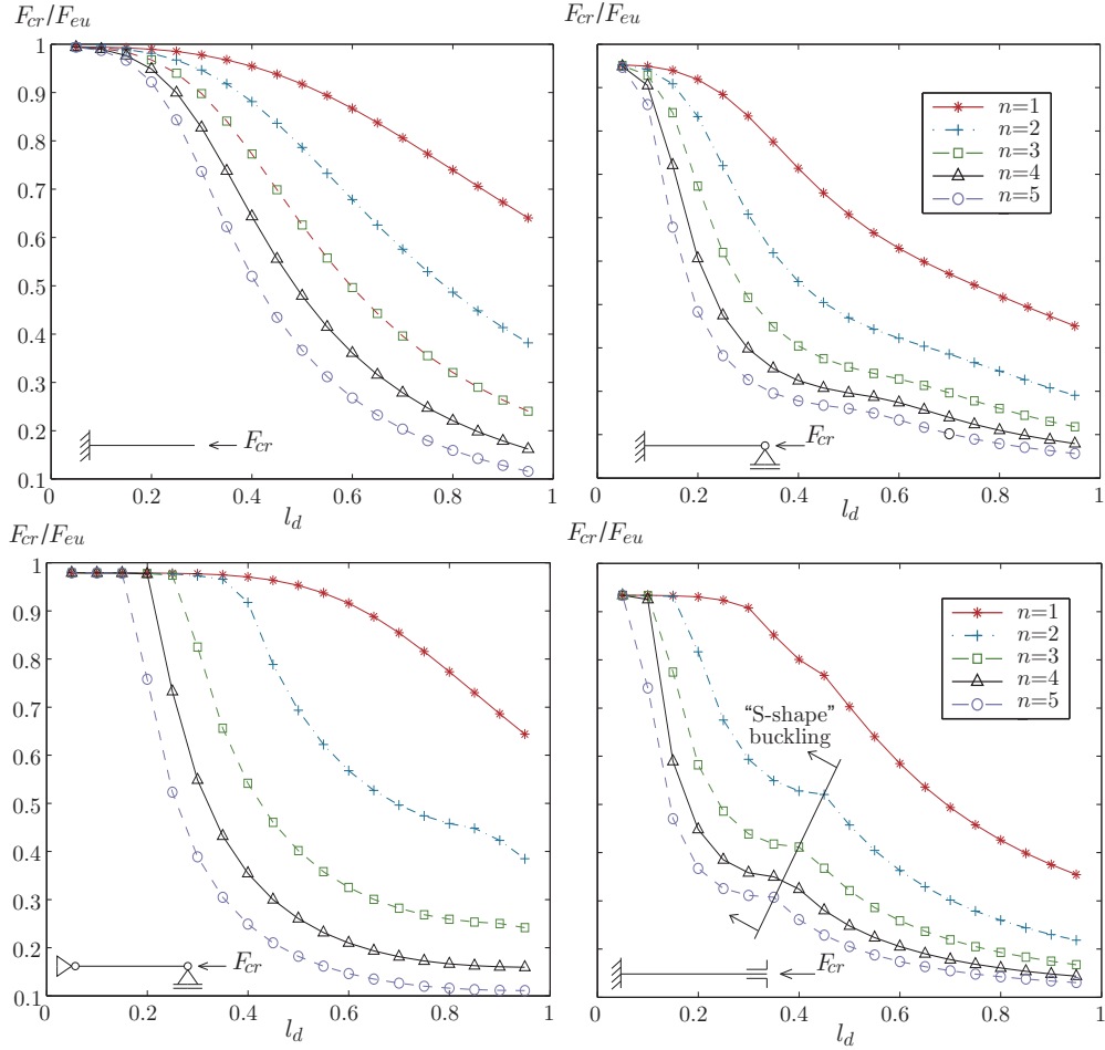
Fig. 10. Normalized buckling load vs. number of delaminations for several delamination lengths.
