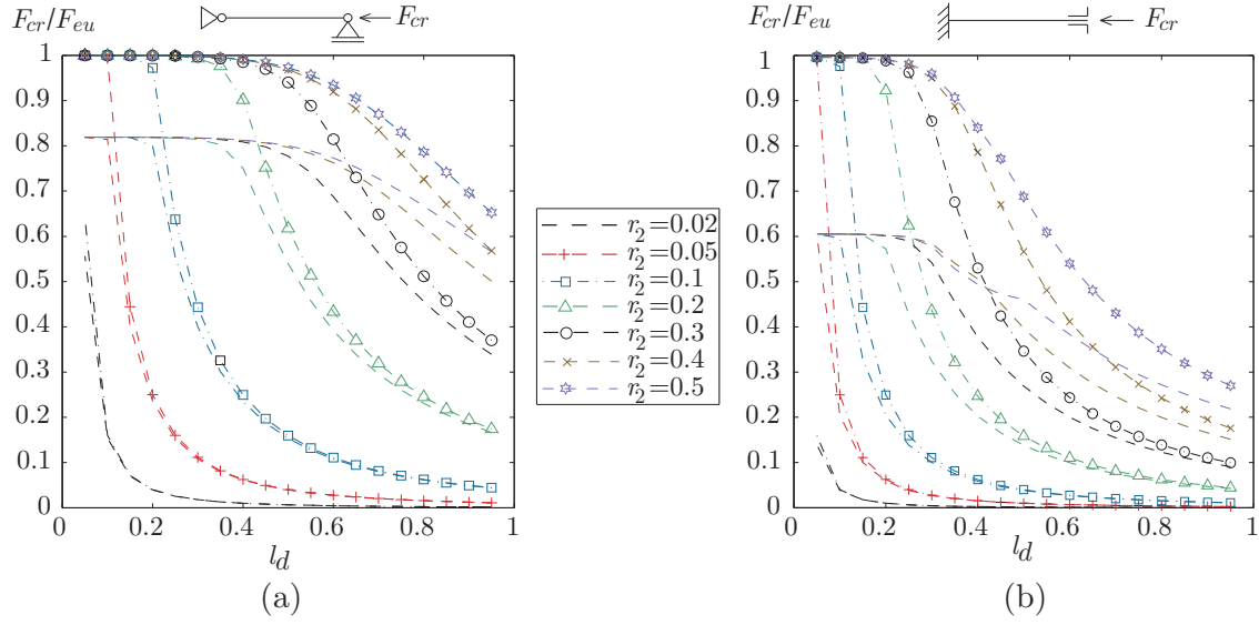
Fig. 4. Normalized buckling loads for (a) simply supported and (b) clamped-clamped beam with a single delaminator vs. delamination length l_d for various relative positions of delamination r_d and two shear moduli G = E/6 (dashed) and G = \infty (marked).
