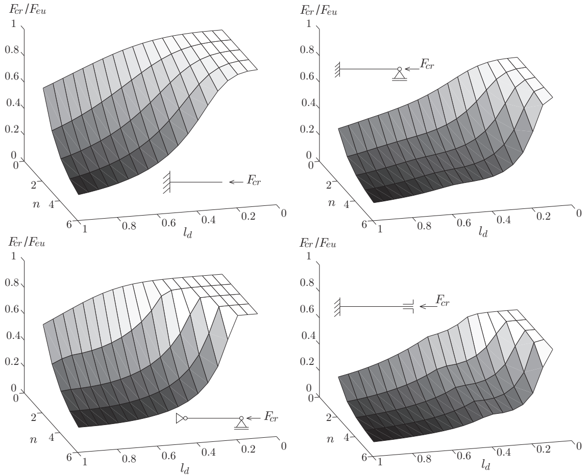
Fig. 11. Normalized buckling load vs. length of delamination l_d and number of delaminations.
