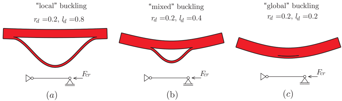
Fig. 5. Buckling shapes for simply supported beam with single delaminator for various delamination lengths, l_d .
