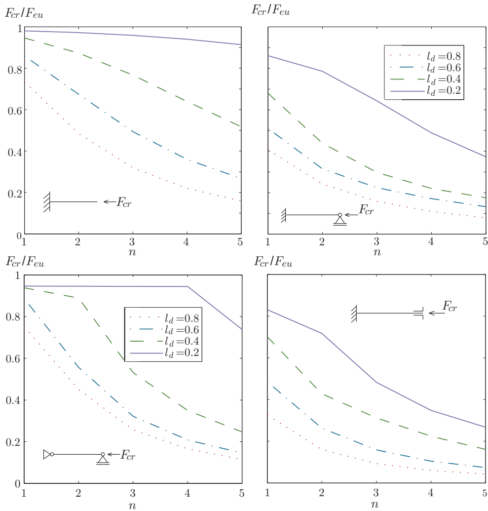
Fig. 9. Normalized buckling load vs. number of delaminations, n , for various lengths of delaminations, l_d .
