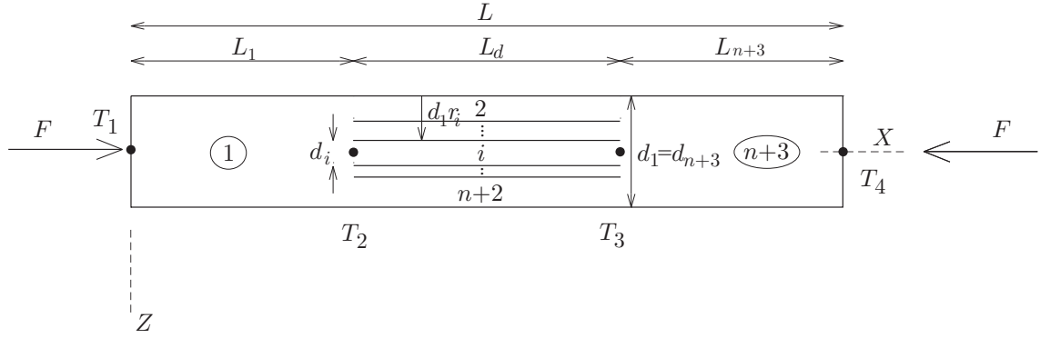
Fig. 1. Model of a multi-delaminated beam with n delaminations.
