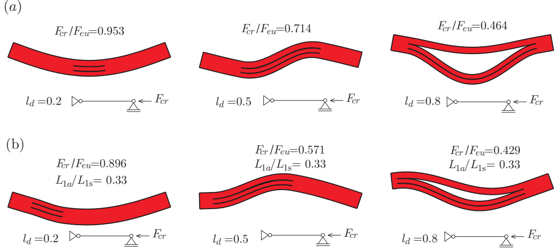
Fig. 12. Buckling shapes and normalized buckling forces for the simply-supported beam with two delaminations for various lengths, l_d . (a) symmetrical delamination; (b) asymmetrical delamination.
