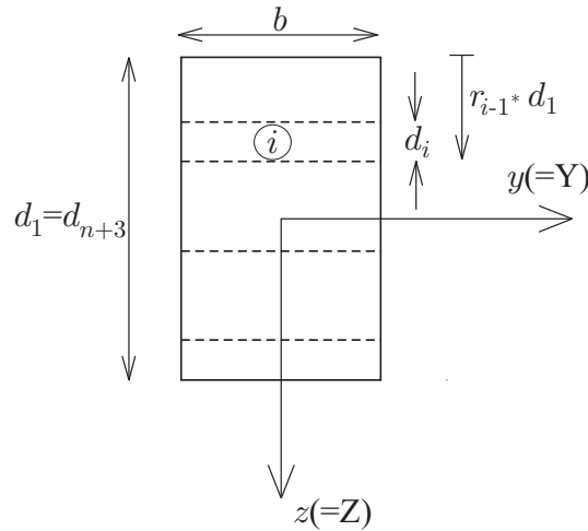
Fig. 2. The cross-section of a delaminated beam with multiple delaminations.
