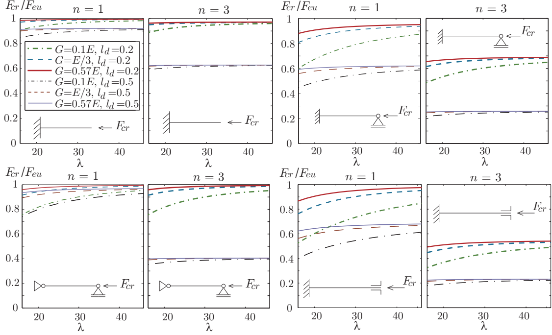
Fig. 8. Normalized buckling load vs. slenderness \lambda for beams with one and three delaminations, for various shear-to-elastic modulus ratios and two delamination lengths, l_d = 0.2 and 0.5 .
