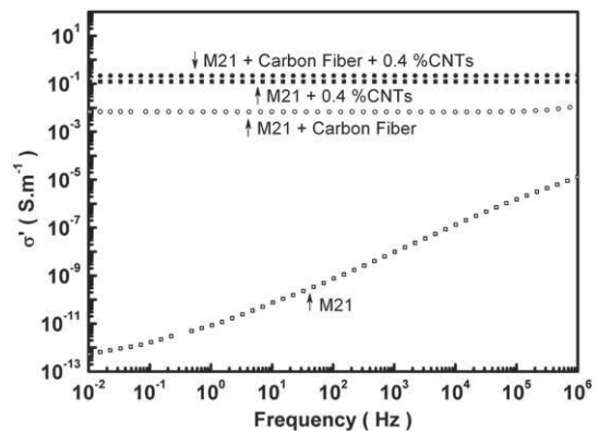
Fig. 2. Frequency dependence of the real part \sigma' of the complex conductivity for M21 epoxy resin ( \square ), carbon fiber composite ( \circ ), M21 epoxy filled with CNTs ( \blacksquare ) and carbon fiber composites with M21 epoxy resin filled in CNTs ( \bullet ).
