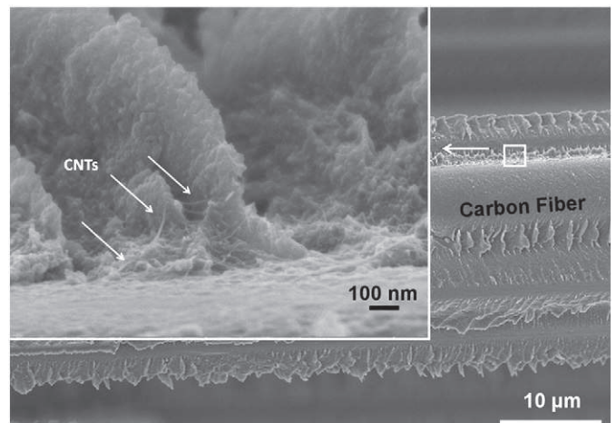
Fig. 5. SEM image of carbon fiber surface of carbon fiber reinforced epoxy filled with CNTs composite. The selected area shows the direct contact between CNTs dispersed in M21 epoxy matrix and carbon fiber embedded in this matrix.
