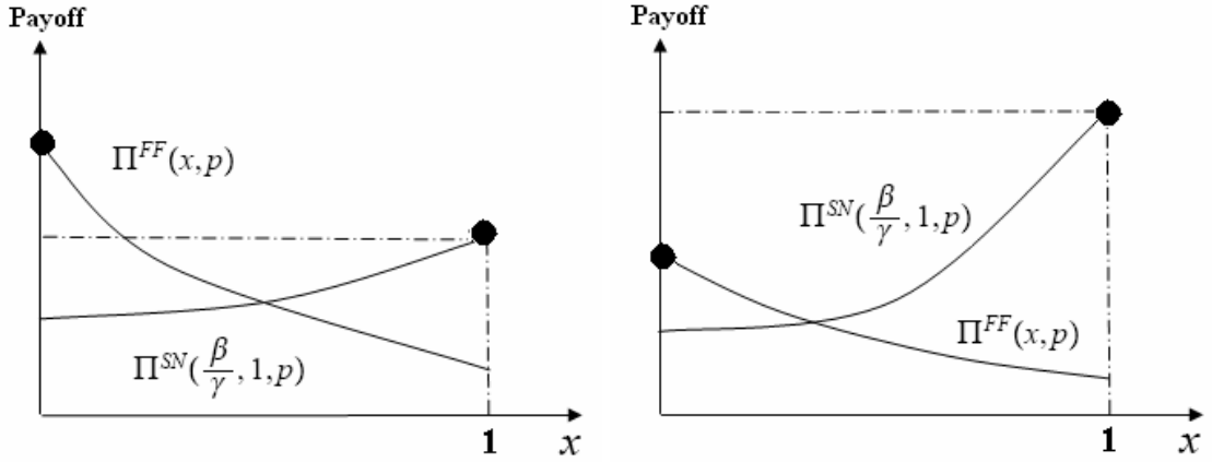
Figure 3: (a) Stationary state (0,0) Pareto dominates \left(\frac{\beta}{\gamma}, 1\right) ; (b) Stationary state \left(\frac{\beta}{\gamma}, 1\right) Pareto dominates (0,0) .
