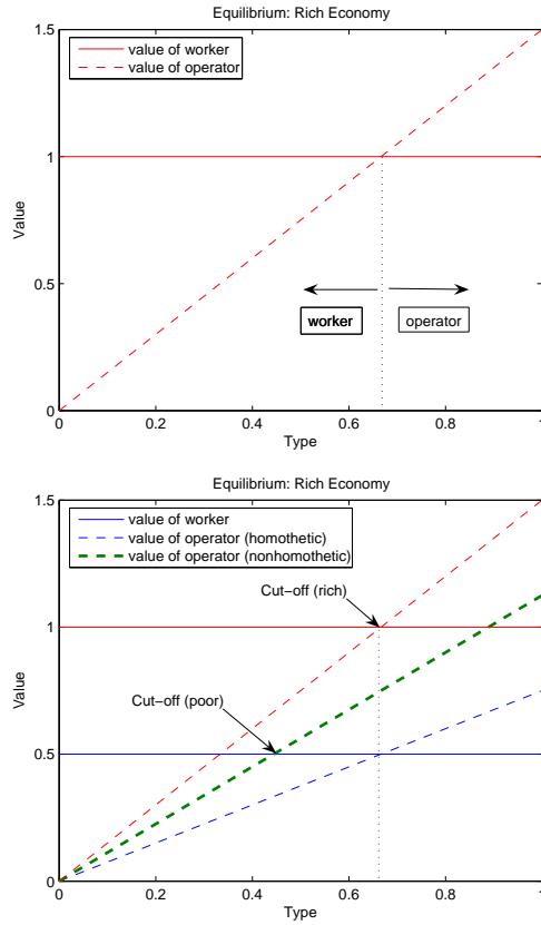
Figure 3: Illustration of Equilibrium Occupation Choice
