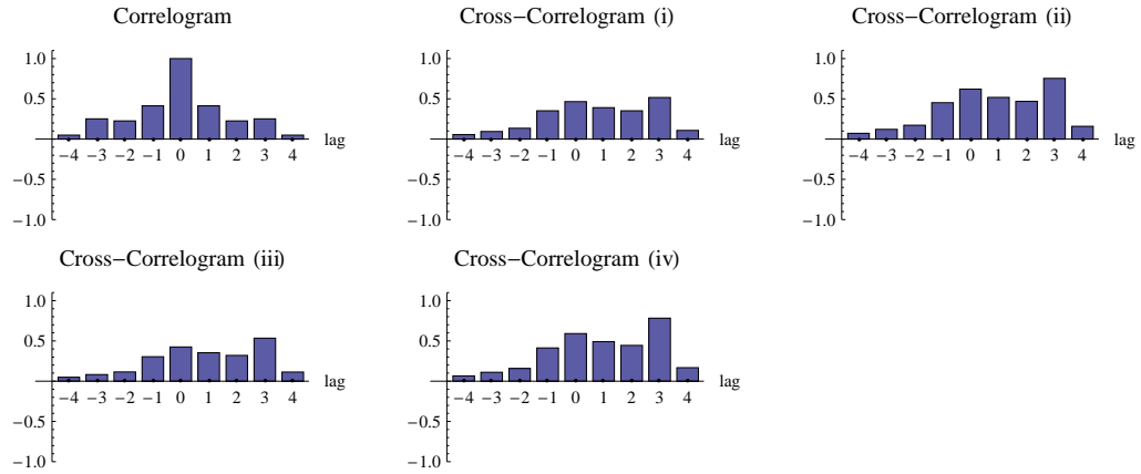
Figure 5: Second moments for DGP - Correlogram of \Delta x_t and cross-correlogram of (\Delta x_t, z_{i,t}) : (i) Leading-Low Corr.-3 Indicators , (ii) Leading-High Corr.-3 Indicators , (iii) Leading-Low Corr.-10 Indicators , (iv) Leading-High Corr.-10 Indicators . Quarterly Data.
