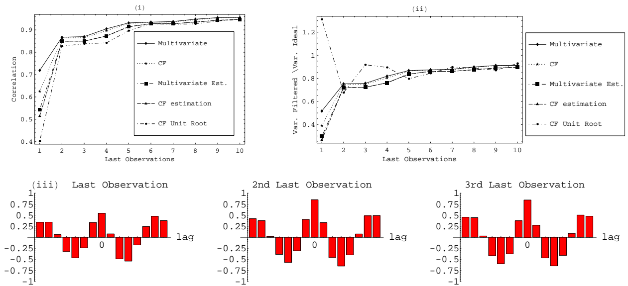
Figure 6: (i) Correlation with ideally filtered series, (ii) variance as proportion of the variance of the ideally filtered series and (iii) cross-correlation function between Multivariate filtered and ideally filtered series. Leading-Low Corr.-3 Indicators , [2, 8] periods band.
