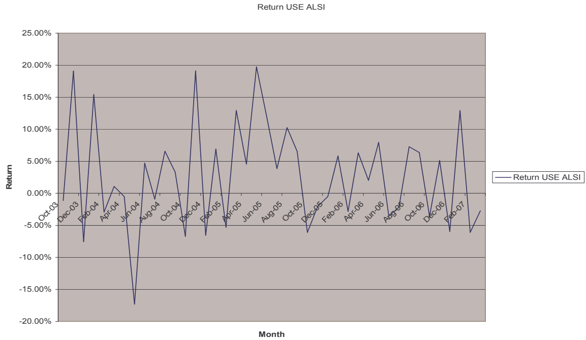
Graph 4.2: USE ALSI holding period return monthly
