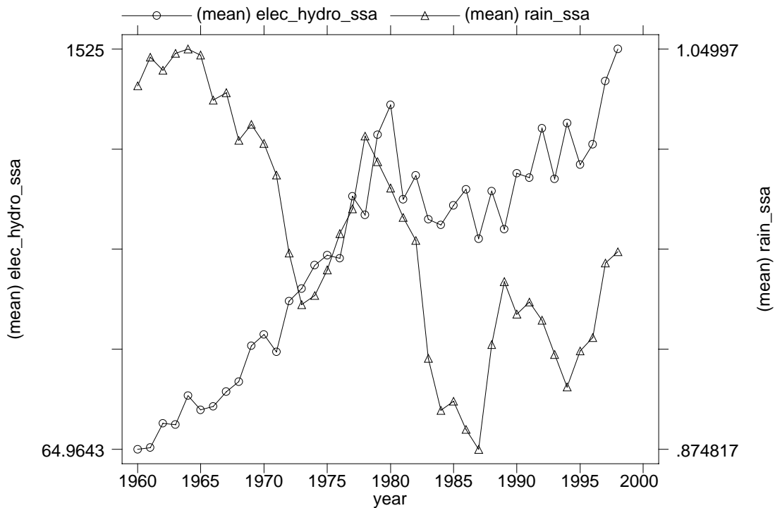
Figure 8: Trends in Hydro-Power Energy Production and Rainfall in SSA
