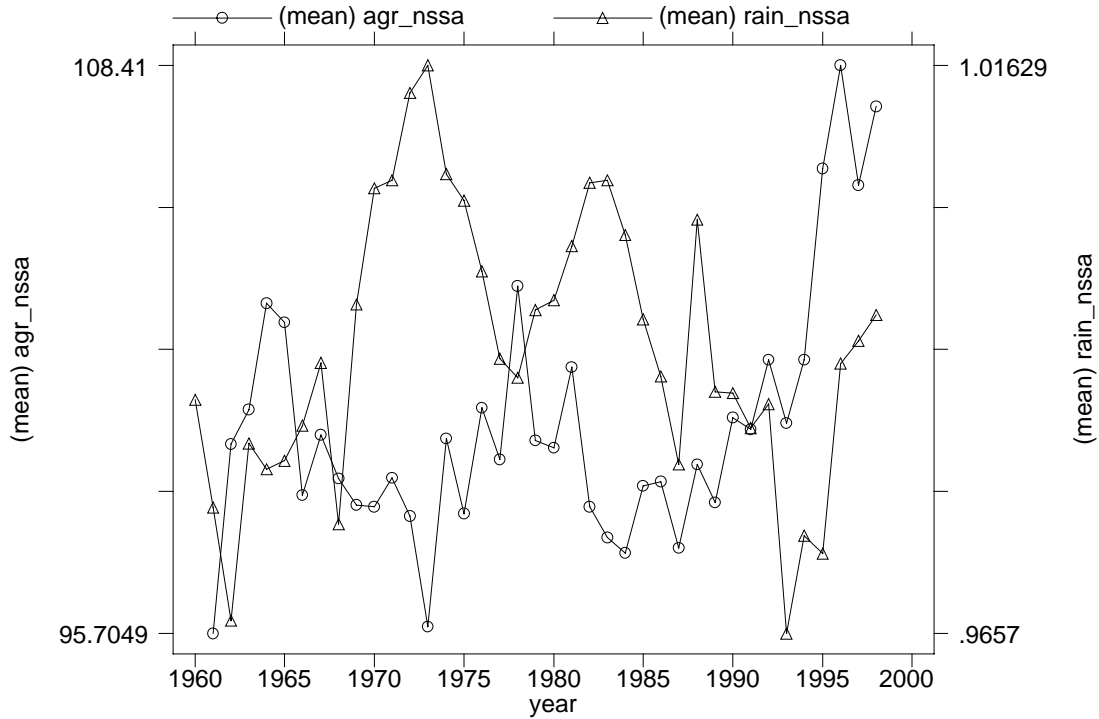
Figure 7: Trends in Agricultural Production and Rainfall in NSSA
