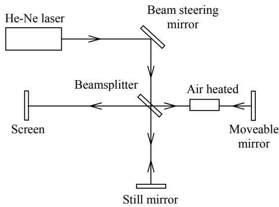
Figure 4. Detecting air temperature at one arm of a Michelson interferometer
