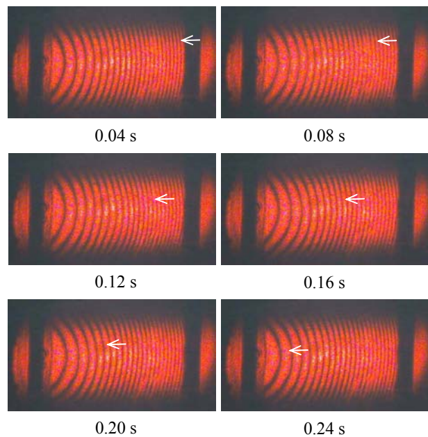
Figure 7. Plasma expansion detected at one arm of the interferometer.
