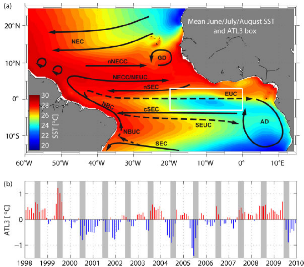
Figure 1. Mean June/July/August SSTs (averaged from 1998 to 2009) in the tropical Atlantic (a). Also included are the main surface (solid) and thermocline (dashed lines) current bands: North Equatorial Current (NEC), North Equatorial Undercurrent (NEUC), North Equatorial Countercurrent (NECC), its northern branch (nNECC), Equatorial Undercurrent (EUC), South Equatorial Current (SEC), its northern and central branches (nSEC, cSEC), South Equatorial Undercurrent (SEUC), North Brazil Current and Undercurrent (NBC, NBUC), as well as the cyclonic circulations around the Guinea and Angola Domes (GD, AD). The white box in (a) defines the region for the ATL3 SST index shown in (b). Monthly SST residuals are calculated by subtracting the mean seasonal cycle; gray bars highlight boreal summer (June/July/August). The microwave optimally interpolated (OI) SST dataset used here is available at www.remss.com .
