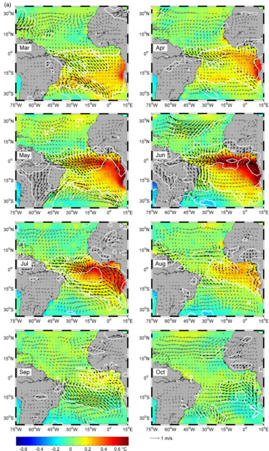
Figure 4. Regression maps of SSTs (color shading) and winds (gray and black arrows) onto the ACT onset (a) and the WAM onset (b) shown in Figure 3. Regressions are calculated separately for the different months from March to October. Significant correlations (95%) between onset dates and SSTs are marked by thick white dashed lines and between onset dates and winds by thin white solid lines and black arrows. SST and wind datasets are HadISST1.1 (Rayner et al., 2003) and NCEP1 (Kalnay et al., 1996), respectively.
