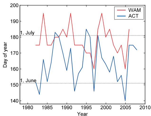
Figure 3. Onset dates for WAM (from Fontaine and Louvet, 2006; obtained using the GPCP dataset) and ACT defined as the date when the surface area, where the SST is below 25°C inside the domain 30°W–12°E and 5°S–5°N, exceeds the empirically fixed threshold of 0.4 \times 10^6 km 2 .
