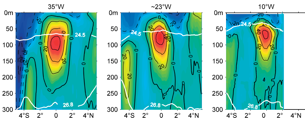
Figure 2. Mean zonal velocity [color shading and black contours (cm/s)] and potential density surfaces 24.5 and 26.8 (white solid lines) along three meridional sections: 35°W, ~23°W, and 10°W (after Brandt et al. , 2006; Hormann and Brandt, 2007; Kolodziejczyk et al. 2009).
