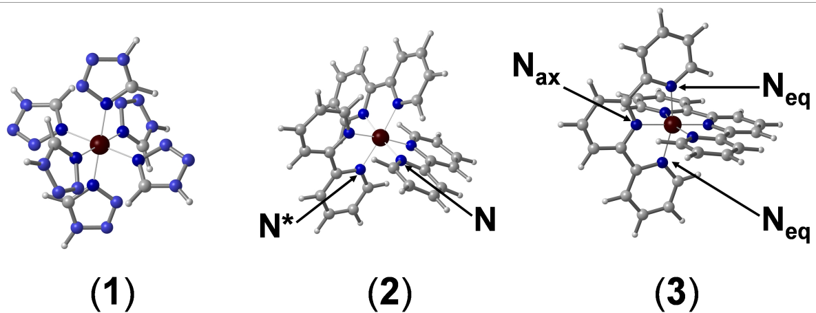
Figure 2. 3D representation of the studied iron complexes: [\text{Fe}(\text{tz})_6]^{2+} ( 1 ), [\text{Fe}(\text{bipy})_3]^{2+} ( 2 ) and [\text{Fe}(\text{terpy})_2]^{2+} ( 3 ). For 2 , we show the notation for N and N* on two neighbouring bipy units, whereas for 3 , we denote the axial and equatorial N positions of a ligand (color online).
