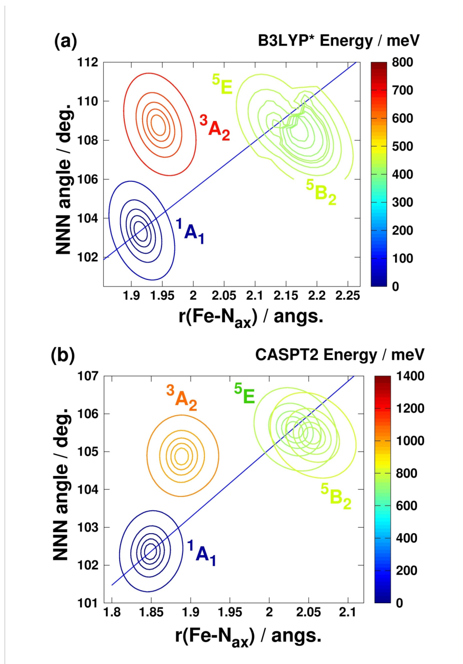
Figure 7. (a) B3LYP* and (b) CASPT2-calculated PESs for the lowest-lying singlet, triplet and quintet states. The zero value of the energy scale is set to the minimum of the ^1A_1 surface. The blue lines represent the combined coordinates for the calculation of 1D potentials. CASPT2 and DFT-calculated energies were splined with a 2D cubic interpolation routine. Contour lines were drawn at the 2,5,10, 20 and 50 meV energy values from the minimum of the corresponding PES. (color online)
