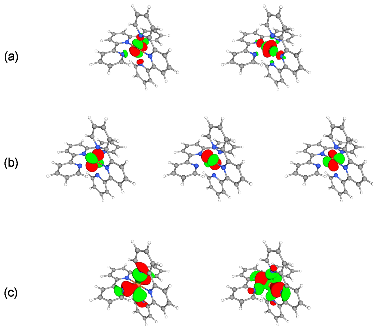
Figure 3. 3D representation of the (a) Fe 3d- e_g antibonding, (b) Fe 3d- t_{2g} non-bonding and (c) Fe-N 2p- e_g bonding active orbitals applied in the multiconfigurational treatment of [\text{Fe}(\text{terpy})_2]^{2+} . For simplicity, the additional set of 4d active orbitals (3 t_{2g} and 2 e_g ) is not shown (color online).
