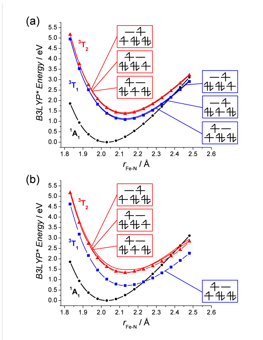
Figure 5. TD-B3LYP*/TZVP calculated triplet states for 1 when invoking the corresponding excitations on a (a) singlet and (b) triplet reference state. The electron configurations corresponding to the individual triplet states are schematically represented in an octahedral ligand field (note that for the sake of simplicity in case of (b) we do not show spin-polarized energy levels). For a better contrast, the ^1A_1 ground state potential is also shown. The zero value of the energy scale is set to the minimum of the ^1A_1 potential (color online).
