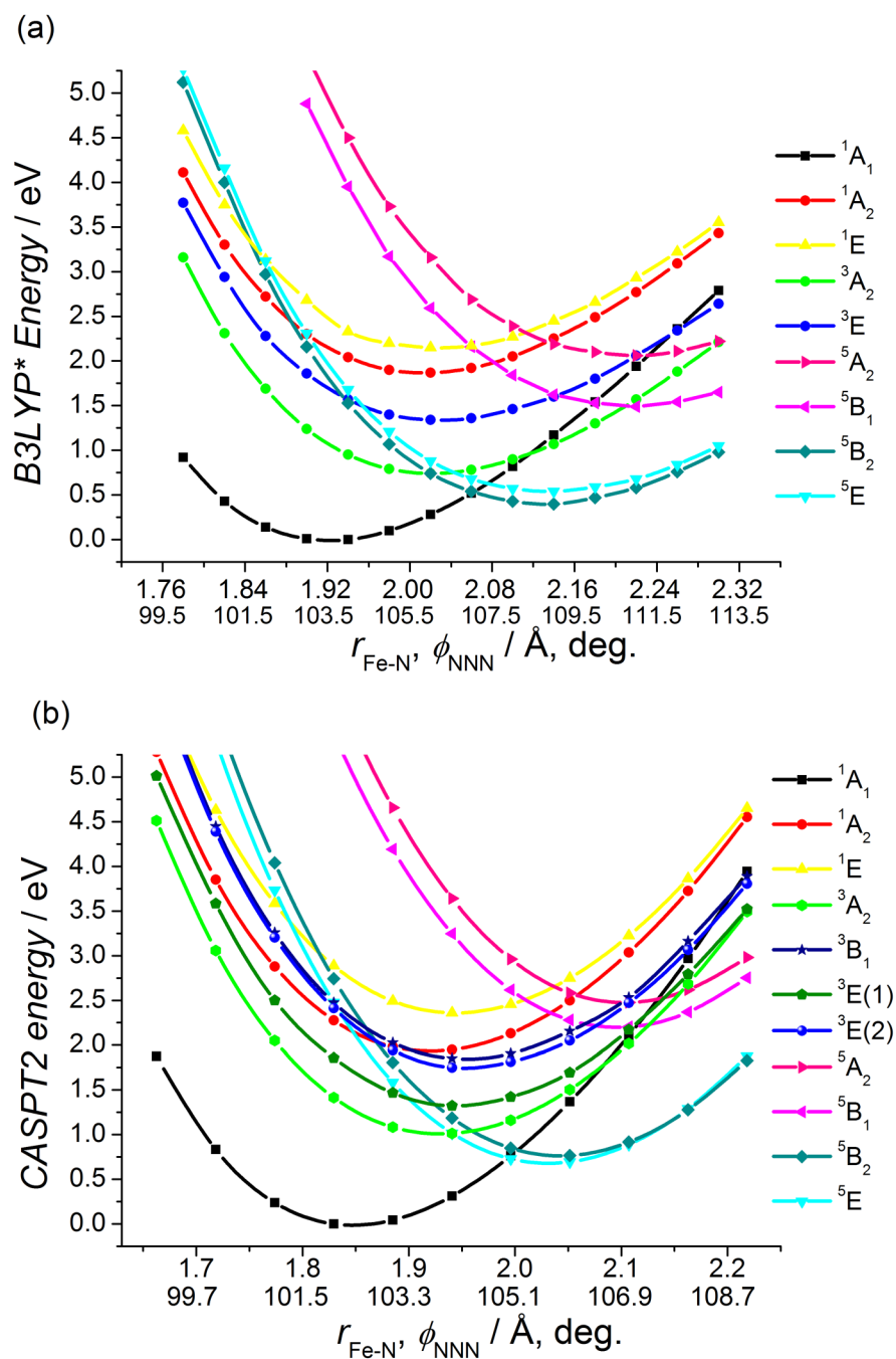
Figure 6. (a) TD-B3LYP* and (b) CASPT2-calculated PESs for [\text{Fe}(\text{terpy})_2]^{2+} ( 3 ) along a combined coordinate, which connects the LS and HS minima. (In case of (a), the triplet states were computed using a triplet reference state.) The notation for each calculated state refers to the D_{2d} point group symmetry. The zero value of the energy scale is set to the minimum of the {}^1\text{A}_1 potential (color online).
