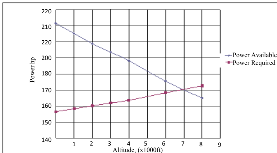
Figure 4: Power Required For Hovering Versus Altitude
