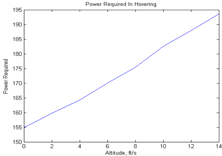
Figure 9: Hovering Power Graph plotted from Matlab
