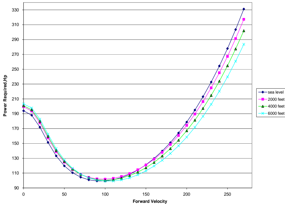
Figure 6: Power Required for Forward Flight versus Velocity at Different Altitude
