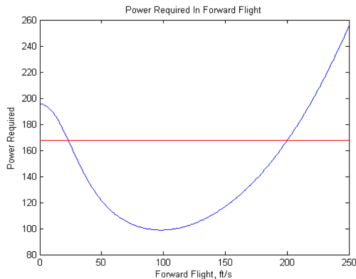
Figure 8: Forward Flight Power Graph plotted from Matlab
