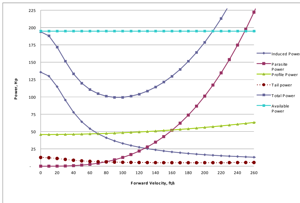
Figure 5: Power Required for Forward Flight versus Velocity
