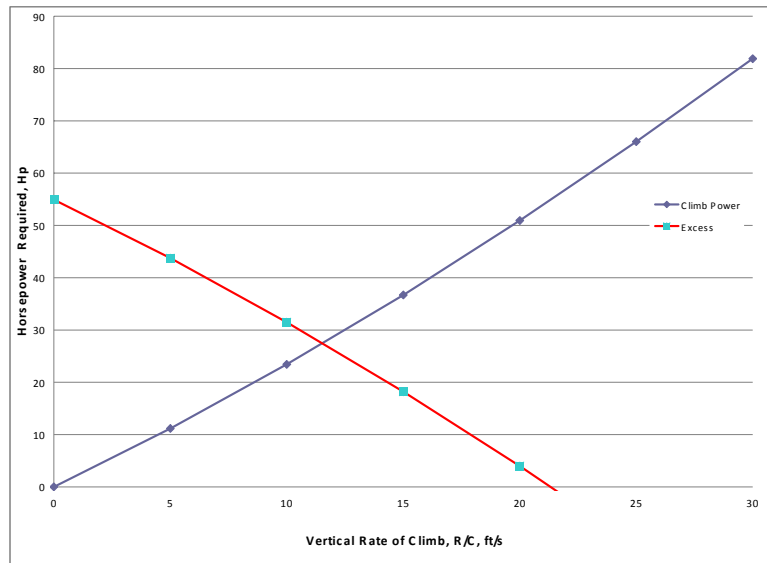
Figure 7: Graph Power Required Versus Climb Rate
