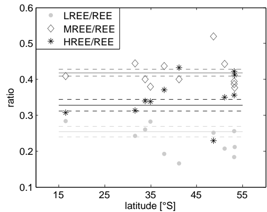
Fig. 9. Ratios between light, medium and heavy REE with latitude in South America: Horizontal lines give the mean glacial values with 1\ \sigma standard deviation (dashed line) (upper line MREE/REE, middle line HREE/REE and bottom line LREE/REE).
