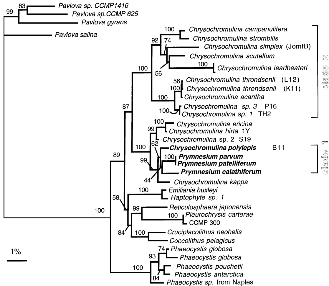
Fig. 1. Molecular phylogenetic tree inferred from the SSU rRNA gene from the Prymnesium/Chrysochromulina group using the neighbour-joining method (redrawn from Medlin et al. , 1997). Strain origins for Chrysochromulina spp. and Prymnesium spp. are as in Table 1. Numbers above the nodes represent percentages of 100 bootstrap repetitions (Felsenstein, 1985).
