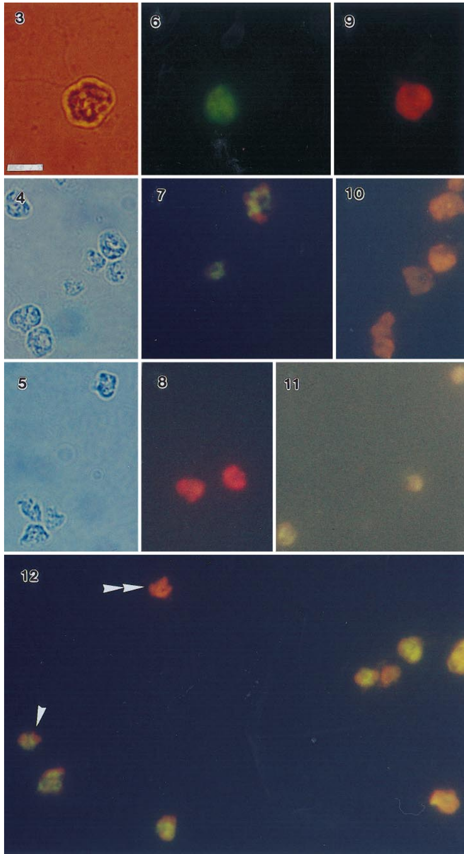
Figs 3–12. Hybridization of the rRNA-based probes CLADE1 and CLADE2 labelled with FLUOS to different Chrysochromulina/Prymnesium . Cells were visualized by light (Figs 3–5) or epifluorescence microscopy (Figs 6–12). Scale bar represents 10 \mu\text{m} and applies to all figures. Positive label of the FLUOS probe appears green, autofluorescence of the cells is red. Figs 3–5. Prymnesium parvum , Chrysochromulina polylepis and C. thronsdonii , respectively, after fixation and incubation in hybridization buffer. Figs 6–8. Prymnesium parvum , Chrysochromulina polylepis and C. thronsdonii , respectively, after incubation in hybridization buffer with the probe CLADE1. Figs 9–11. Prymnesium parvum , Chrysochromulina polylepis and C. thronsdonii , respectively, after incubation in hybridization buffer with the probe CLADE2. Fig. 12. Mixture of both C. polylepis (simple arrowhead) and C. thronsdonii (double arrowhead) hybridized with the probe CLADE1.
