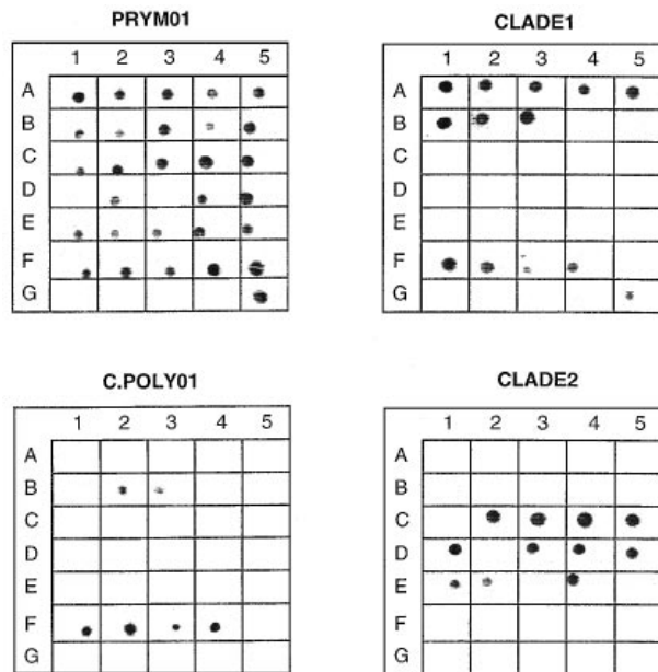
Fig. 2. Dot-blot hybridization of filter bound DNA (amplified SSU rRNA gene) with the digoxigenin-labelled oligonucleotide probes PRYM01, CLADE1, CPOLY01 and CLADE2. The grid shows the following members of the Chrysochromulina / Prymnesium group. A-1, -2, -3; Prymnesium patelliferum (K-0252, PCC 527, RH pat 93); A-4, -5, B-1: P. parvum (K-0081, RC 10 parv 93 and PCC 94); B-2, -3, F-1, -2, -3, -4: Chrysochromulina polylepsis (clones S, B11, CCMP 287, PCC 200, A and K, respectively); B-4: C. kappa ; B-5, C-1: C. hirta (clones 1Y and PN2-14); C-2: C. campanulifera ; C-3, -5: C. cf. strobilus ; C-4: C. cf. simplex , D-1, -3: C. leadbeateri ; D-2: C. ericina ; D-4: C. thronsdensii ; D-5, Chrysochromulina sp. 1 (TH2); E-1: C. scutellum ; E-2; C. acantha ; E-3: Chrysochromulina sp. 2 (S19); E-4: Chrysochromulina sp. 3 (P16); E-5: C. cf. minor ; F-5: C. brevifilum ; G-5: C. chiton . G-1, -2, -3, -4 are empty.
