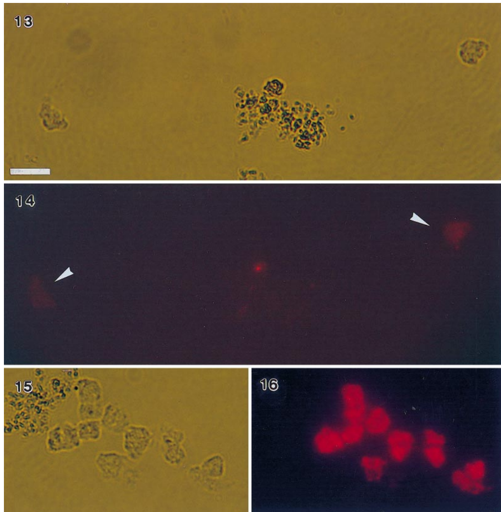
Figs 13–16. Hybridization of the rRNA-based probe CLADE1 labelled with Cy3 to Chrysochromulina polylepis . Scale bar in Fig. 13 represents 10 \mu\text{m} and applies to all figures. Figs 13, 14. Bright field photomicrograph (Fig. 13) and the corresponding field viewed by epifluorescence microscopy (Fig. 14) for a preparation of cells incubated in hybridization buffer without probe, showing autofluorescence of the cells (arrowheads). Positive label of the Cy3 probe is bright red (Fig. 16) in comparison to the paler red autofluorescence of the cells (Fig. 14). Figs 15, 16. Cells hybridized with CLADE1 labelled with Cy3 visualized by light microscopy (Fig. 15) and showing strong fluorescence with epifluorescence microscopy (Fig. 16).
