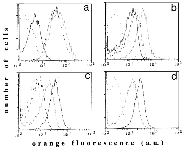
Fig. 17. Histograms (number of cells vs orange fluorescence) obtained from the analysis of cell populations of (a) Chrysochromulina polylepis , (b) Prymnesium parvum (c) C. leadbeateri and (d) C. acantha by flow cytometry. Number of cells were standardized for clarity (Y axis). A. u. represents arbitrary units (X axis). Cells were fixed, permeabilized and incubated either without probes (autofluorescence of cells, . . . .) or with CY3-labelled CLADE2 (—), CLADE1 (.....) and CPOLY01 (----). When cells are positively labelled with a probe there is an increase in the intensity of the fluorescence signal as detected by the flow cytometer. With maximum separation of labelled and non-labelled/non-specific labelled populations, the histograms have minimum overlap. For example, in panel A, C. polylepis is labelled equally well by both CLADE1 and CPOLY01 probes with little overlap with CLADE2 probe. The remaining panels show some overlap between target (histogram with the highest fluorescence values) and non-specific labelling.
