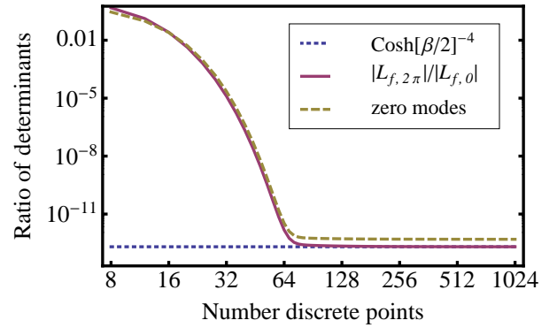
FIG. 6. Ratio of determinants for the phase profile pictured in Fig. 5(a) computed using different methods. (1) following the prescription of Method 1 we integrate out the fermionic degrees of freedom without discretization, and raise the final answer to the fourth power to compensate for the two fermion doublings in the discretized methods (labeled: \cosh(\beta/2)^{-4} ). (2) following prescription of Method 2, we compute the fermion determinants on a discrete lattice (labeled: |L_{f,2\pi}|/|L_{f,0}| ). (3) following Method 2, by constructing the ratio of the four smallest fermion eigenvalues (\lambda_{1,2\pi}/\lambda_{1,0}) \times \dots \times (\lambda_{4,2\pi}/\lambda_{4,0}) of H_{f,2\pi} and H_{f,0} , respectively (labeled: zero modes). Comparison of the three curves indicates that the suppression of tunneling is indeed controlled by the zero modes, with the small offset being a non-universal feature associated with the duration of the phase slip.
