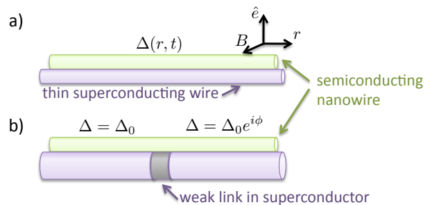
FIG. 3. Schematic of a composite structure consisting of a semiconducting nanowire in contact with a superconductor. The superconductor induces pairing in the nanowire via proximity effect. The orthogonal alignment of the spin-orbit field \hat{e} , the magnetic field B , and the coordinate along the wire r is indicated. In implementation (a) the superconductor is a thin homogenous wire that is susceptible to phase slips along its entire length. In implementation (b) the superconductor is rigid everywhere except a weak link, a point at which phase-slips can occur.
