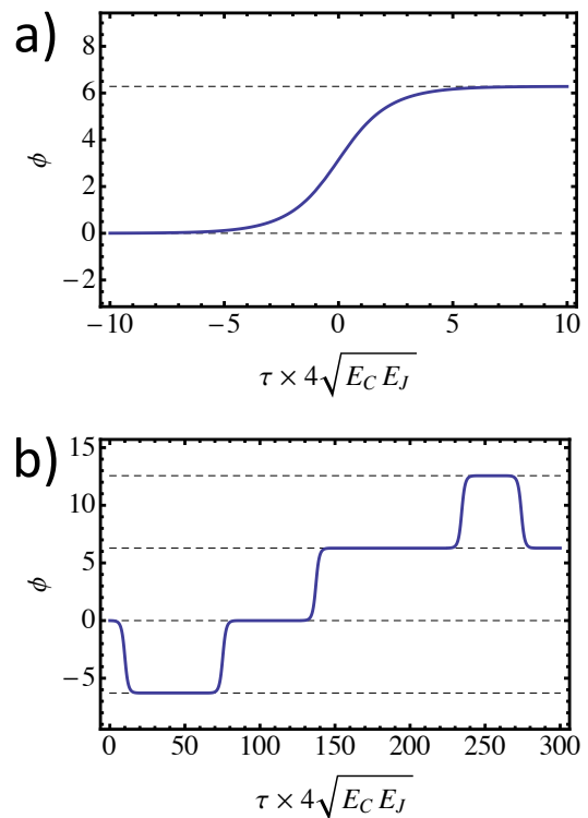
FIG. 4. (a) Instanton trajectory in the sine-Gordon model, Eq. (4). (b) Schematic representation of the dilute instanton gas composed of 2\pi phase slips and -2\pi anti-phase-slips.
