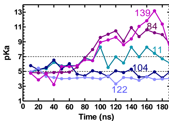
Figure 5 Changes in the pKa values of selected residues during the simulation, calculated using the propKa 3.1 server.
