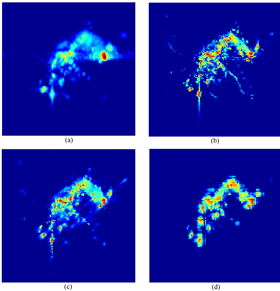
Fig. 4. Results with the AFRL Backhoe data (a) conventional reconstruction (b) point-enhanced nonquadratic regularization (c)-(d) sparse representation based reconstructions : (c) PR dictionary (d) wavelet dictionary
