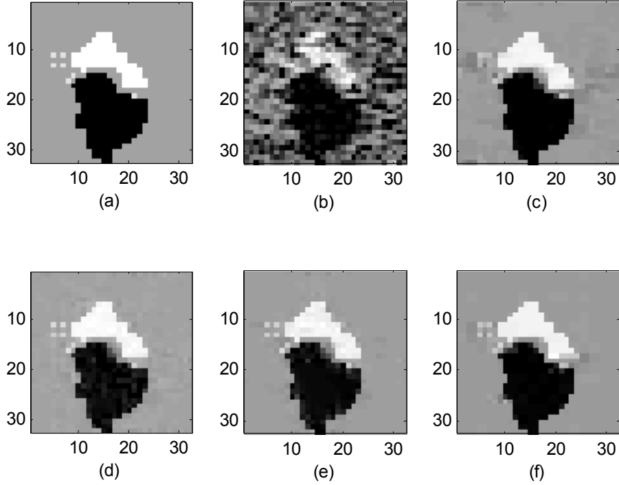
Fig. 2. Synthetic ADTS scene reconstruction (a) synthetic scene (b) conventional reconstruction (c) point-region-enhanced nonquadratic regularization (d)-(f) sparse representation based reconstructions: (d) SB dictionary (e) PR dictionary (f) wavelet dictionary
