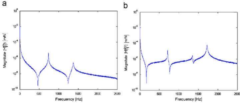
Fig. 4. (a) Distorted tip-point FRF ( H_{11}^{sh} ) of the spindle-holder subassembly and (b) distorted tool point FRF ( H_{11}^{st} ) of the spindle-holder-tool assembly.
