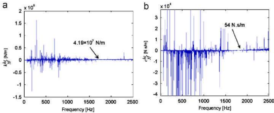
Fig. 5. Dynamical parameters at the holder-tool interface obtained from Eq. (6) by using the distorted FRFs; (a) linear displacement-to-force stiffness k_y^{st} and (b) linear displacement-to-force damping c_y^{st} .
