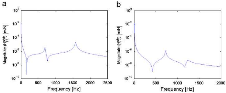
Fig. 2. (a) Analytically obtained tool point FRF ( H_{11}^{st} ) of the spindle-holder-tool assembly and (b) the analytically obtained tip-point FRF ( H_{11}^{st} ) of the spindle-holder subassembly.
