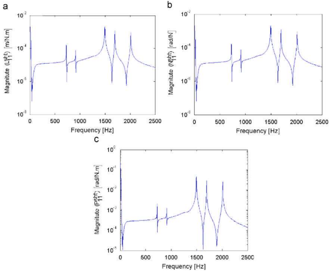
Fig. 9. (a) Approximately obtained tool point FRF ( L_{11}^{ht} ) of the spindle-holder-tool assembly, (b) approximately obtained tool point FRF ( N_{11}^{ht} ) of the spindle-holder-tool assembly and (c) approximately obtained tool point FRF ( P_{11}^{ht} ) of the spindle-holder-tool assembly.
