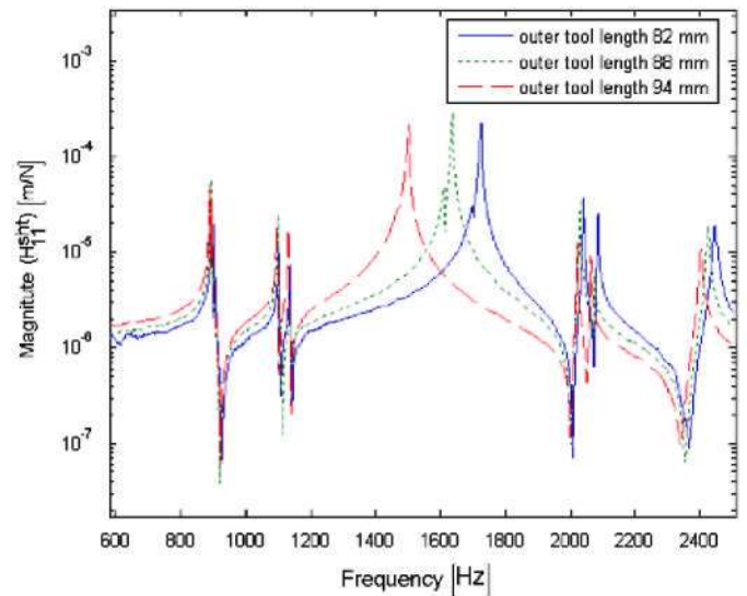
Fig. 10. Tool point FRF with changing tool length outside the holder.
