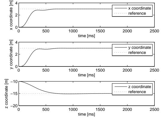
Fig. 4. Position control of the vehicle under no disturbance condition
