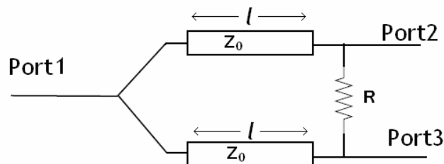
Fig. 1 A transmission line two-way Wilkinson power combiner
