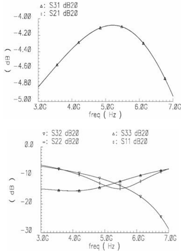
Fig. 6 S-Parameter Simulation Results of impedance matching Wilkinson power combiner
