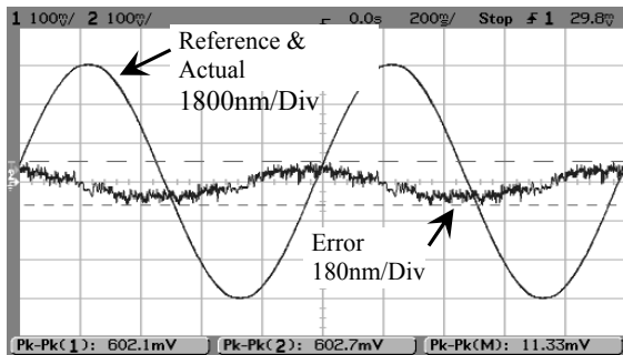
Fig. 7: DSP tracking experiment for 10.8 \mu m pp 1Hz sinusoidal reference.
