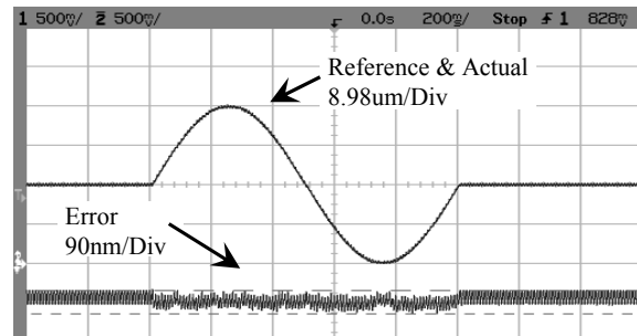
Fig. 9: Tracking of 35.60 \mu m pp 1Hz sinusoidal reference. The error is 54nm pp (0.15%).
