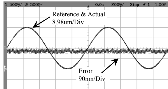
Fig. 8: Tracking of 35.69 \mu m pp 1Hz sinusoidal reference. The error is 50nm pp (0.14%).
