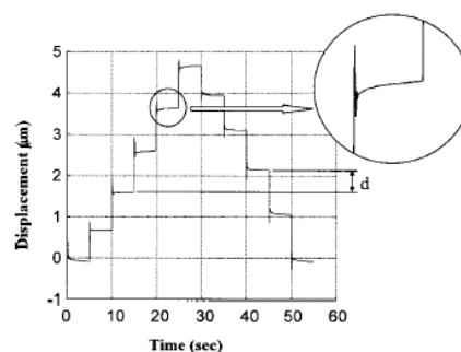
Fig. 1: Open loop step response of the piezoelectric actuator. “d” is the displacement difference due to hysteresis. Creep effect is magnified in the circular view [16].
