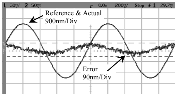
Fig. 6: DSP tracking experiment for 4.5 \mu m pp 1Hz sinusoidal reference.
