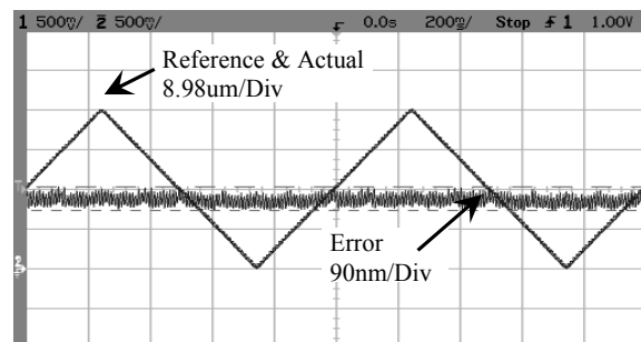
Fig. 10: Tracking of 35.60 \mu m pp 1Hz triangular reference. The error is 54nm pp (0.15%).
