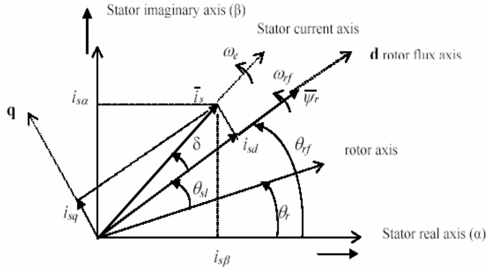
Figure 2.4: Rotor flux and stator current in the stationary ( \alpha - \beta ) and the rotary frame of reference (d-q)
