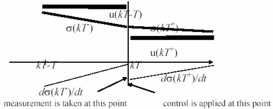
Figure 2.7: The relations between measured and calculated variables for discrete time systems without computational delay
