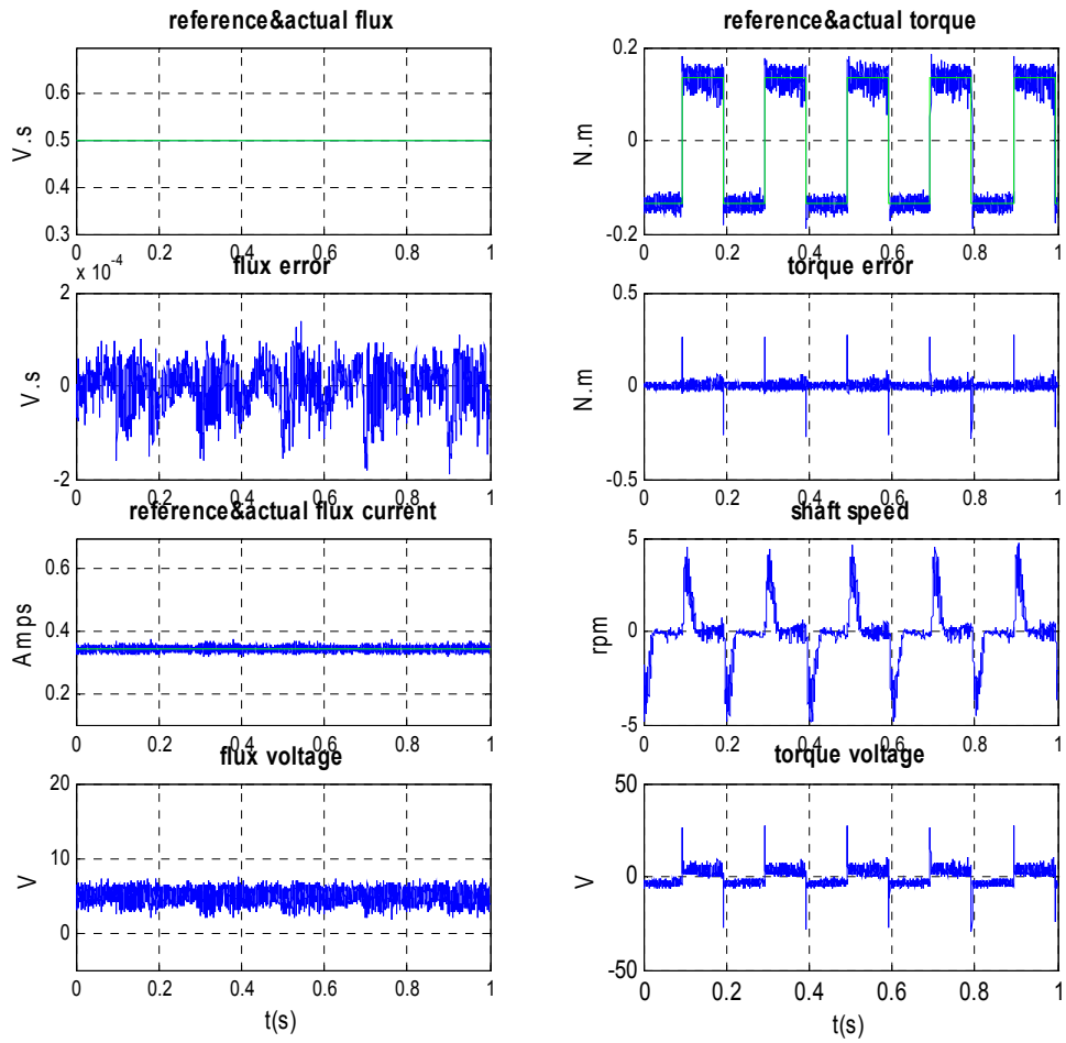
Figure 4.11: 10 Hz pulse torque reference and 0.5 V.s constant flux reference
