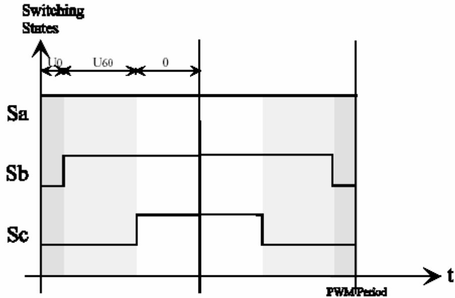
PWM Sstates with 0 \leq \theta \leq 60 deg
