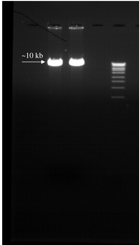
Figure 4.27: 1% agarose gel electrophoresis showing the Hind III digestion of the vector pEGKG. Samples were run at 100 V for 1.5 hours
