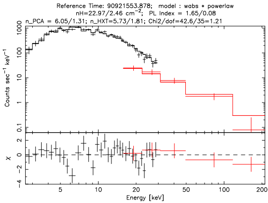
Fig. 2. Spectrum of an SGR 1806–20 burst, detected in 1996, modeled with a power law.
