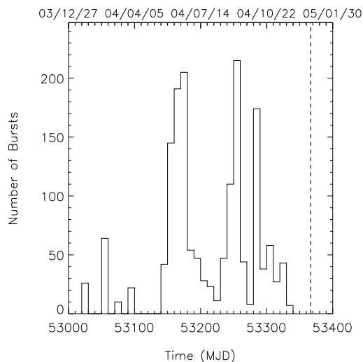
Fig. 1. Burst activity history of SGR 1806–20 within RXTE pointings. The dashed vertical line denotes the time of the giant flare on 27 December 2004.
