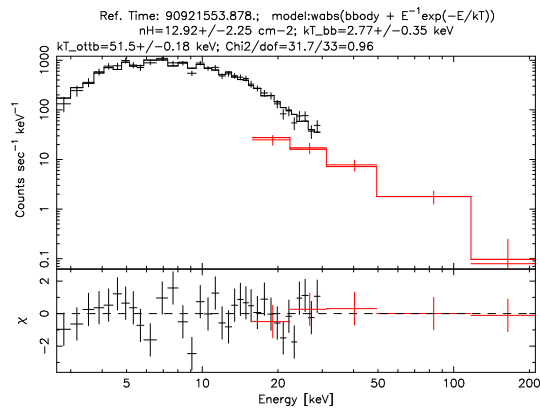
Fig. 3. Spectrum of the same burst as in Figure 2 modeled with the sum of a blackbody and an OTTB models.
