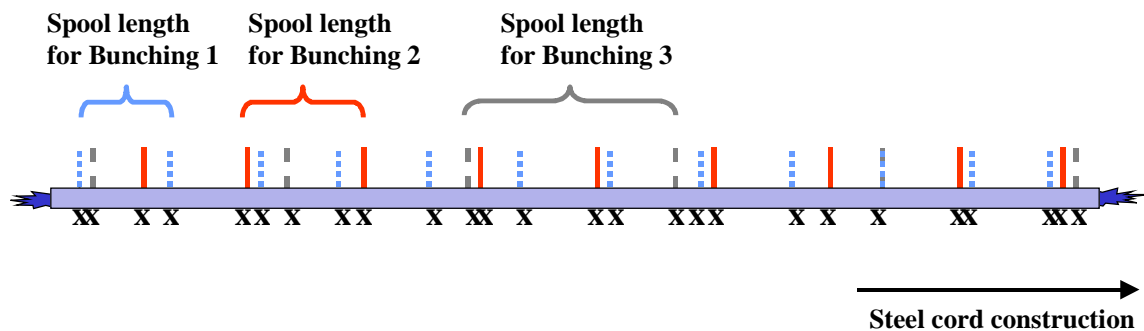
Figure 5: Locations of knots in Case 2. The x signs denote the knots due to change-overs. The intervals shown in brackets correspond to lengths of work-in-process spools, and are decision variables in the simulation model.
