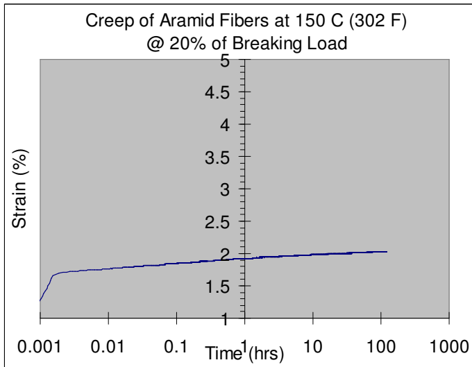
Fig. 4 Creep strength at 150 °C (302 °F).
