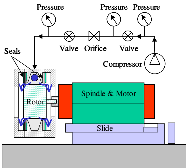
Fig. 7 Subscale dynamic seal test rig
