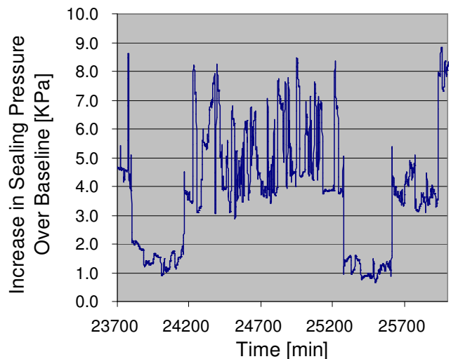
Fig. 10 Field test results for 7EA #1 (inlet) bearing sealing application.
