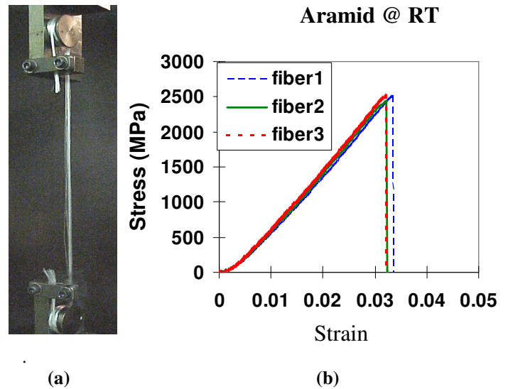
Fig. 1 Tensile tests: a) configuration b) repeatability.
