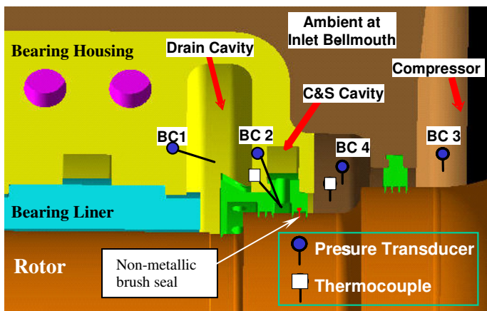
Fig. 9 The 7EA #1 (inlet) bearing sealing application
