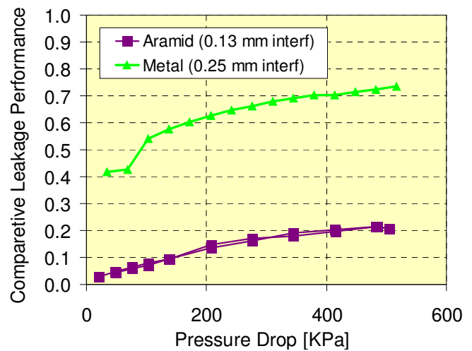
Fig. 8 Sample Aramid Seal Leakage Data
