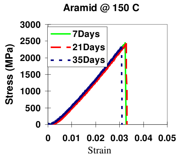
Fig. 2 Fiber strength upon exposure to 150 °C (302 °F).
