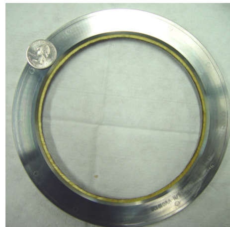
Fig. 6 Subscale aramid fiber brush seal.
