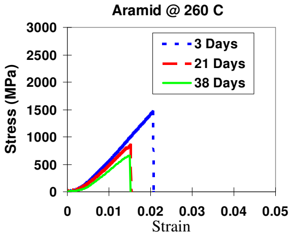
Fig. 3 Fiber strength upon exposure to 260 °C (500 °F).
