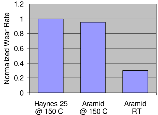
Fig. 5 Wear test results for aramid and Haynes 25 tufts against Ni-Cr-Mo-V. Data are normalized with wear rate of Haynes 25 bristles at 150 °C.
