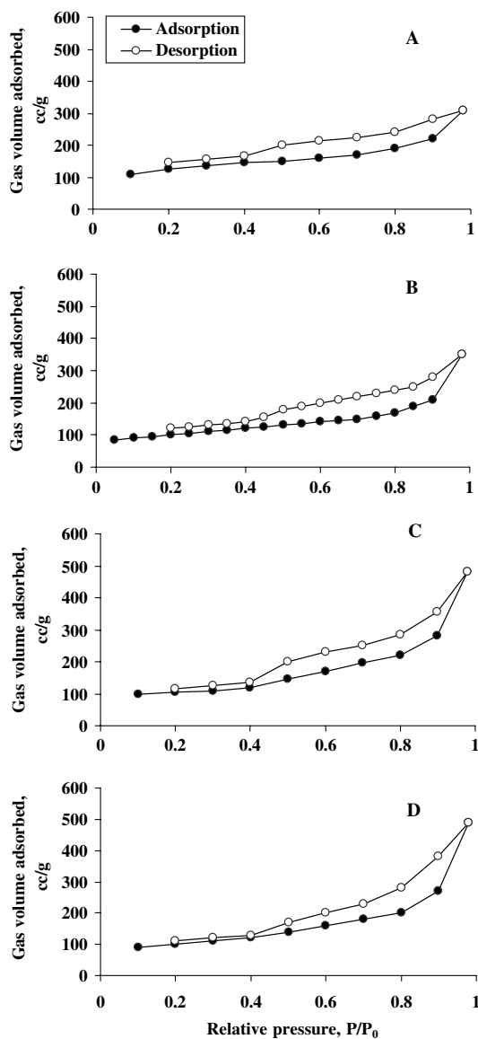
Fig. 4. N_2 adsorption/desorption isotherms of natural zeolite-templated carbons, produced at (A) 700 °C, (B) 800 °C, (C) 900 °C and (D) 1000 °C.
