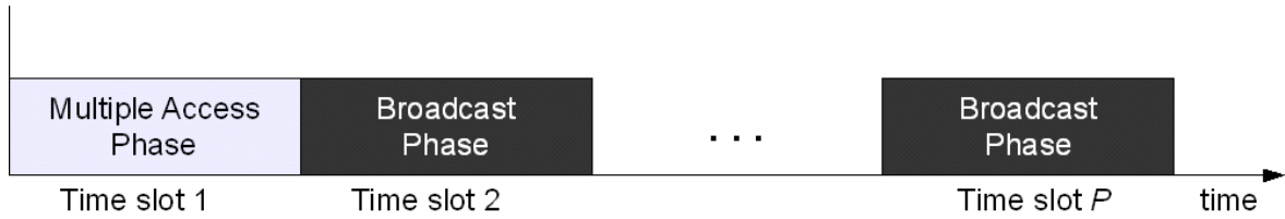
Figure 3.2. Communication protocol for MGMW relaying
