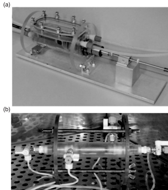
Figure 3. Dual closed-loop perfusion bioreactors by (a) Bilodeau et al. [130], and (b) Zhang et al. [131]. Reproduced with permissions.
