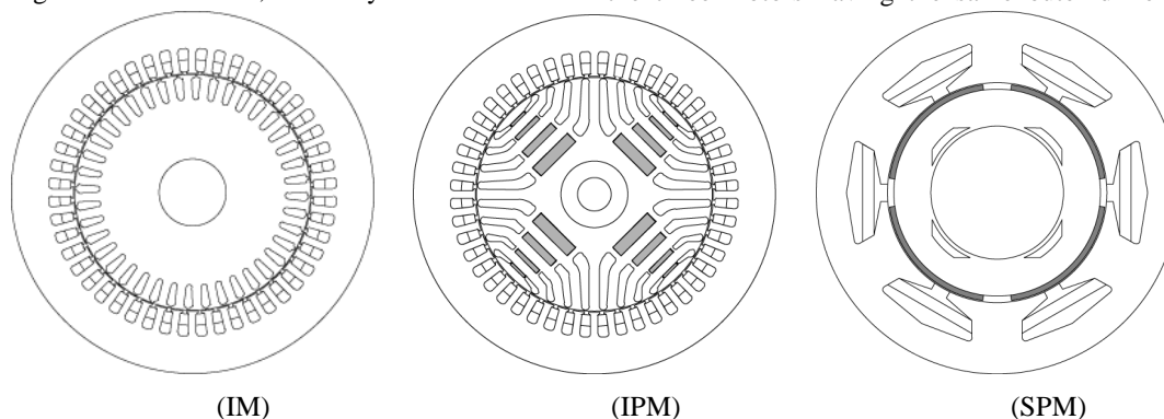
Figure 1. Induction motor, Interior PM motor and Surface mounted PM motor under investigation.
