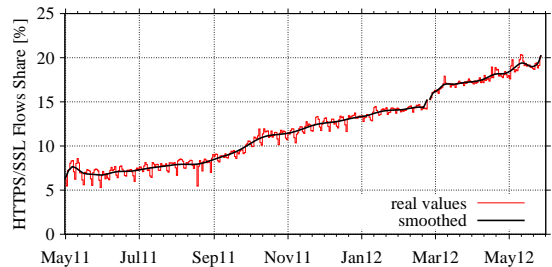
Fig. 2. Evolution of the percentage of HTTPS/SSL connections over 1 year.
