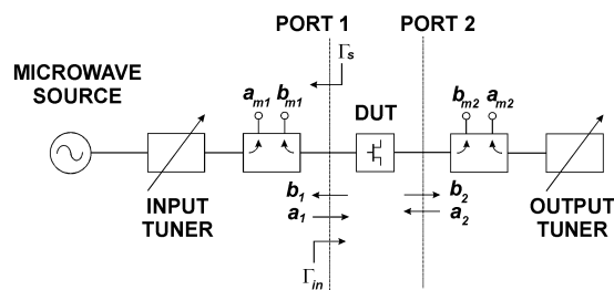
Fig.1. Simplified block scheme of a traditional test-set for both source and load-pull characterization of active devices.
